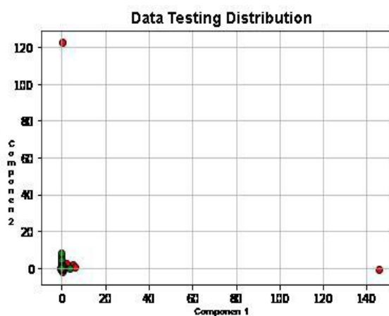
Figure 4. PCA the deployment of testing data
