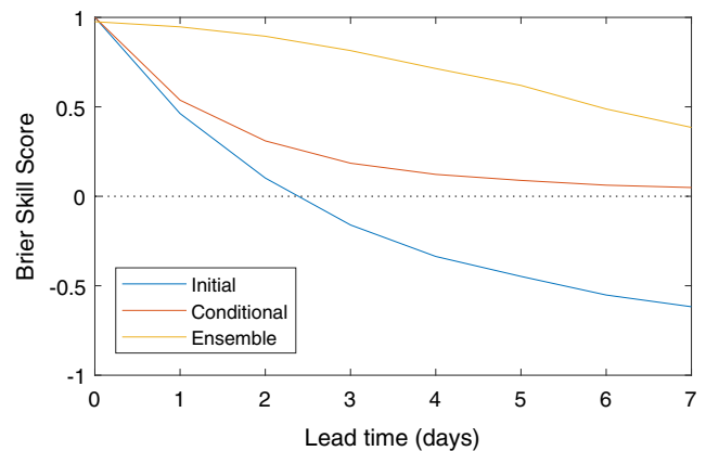
FIGURE 1 Brier skill score relative to climatology for different forecasts of the future weather regime
