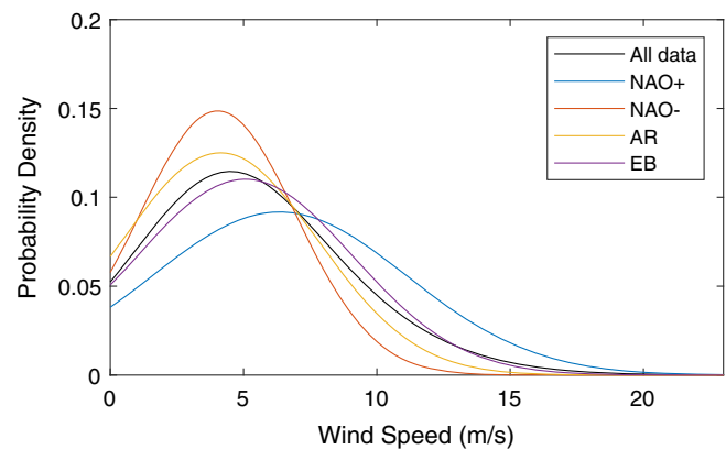
FIGURE 13 Empirical distributions of wind speed at a location close to Bergen, Norway, when each identified regime occurs in the reforecast setting
