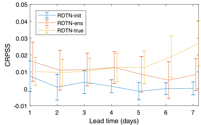
FIGURE 12 CRPSS against lead time for each of the three regime-dependent methods at a location close to Bergen, Norway. Scores for RDTN-ens have been offset by 0.1 days and those for RDTN-true by 0.2 days, to visualise 95% confidence intervals around the scores
