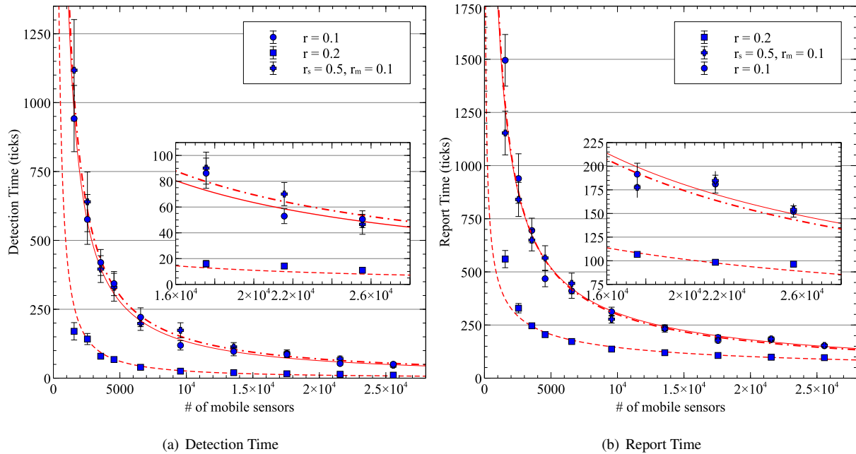
Figure 9: Effect of sensor radius on SNoS performance, when sensors move accordingly to Song’s model. We can increase radius of every sensor, or we can increase only sensor radius r_s of static sensors. Detection time performance is not influenced by an increase in sensor radius of static sensors, unless the event is deployed in their sensing range, which is not the case here.
