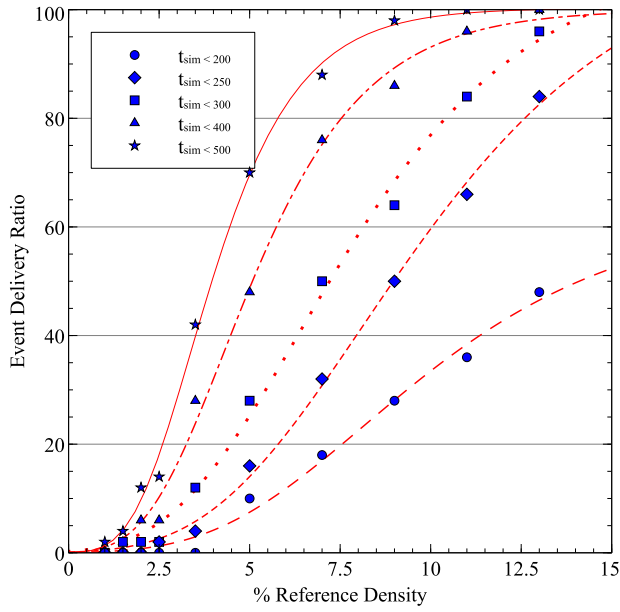
(a) Delivery Ratio of IM model with r = 0.1
