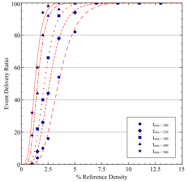
(b) Delivery Ratio of IM model with r = 0.2
