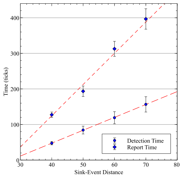
(a) Detection Time and Report Time
