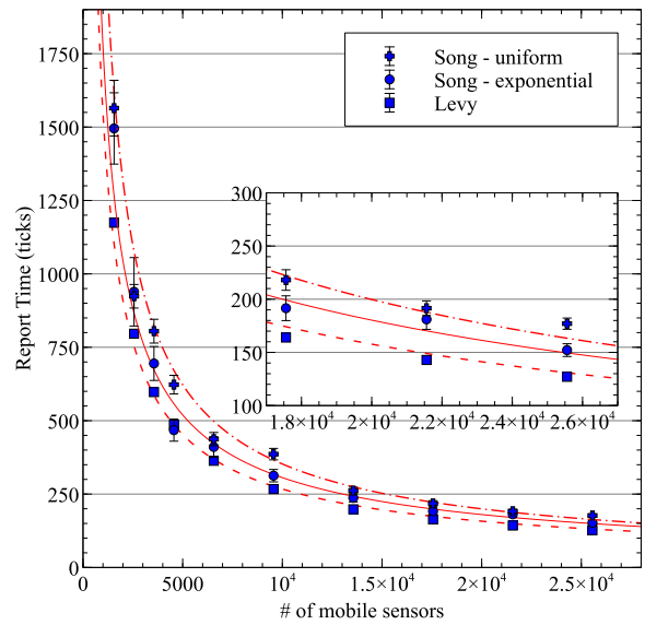
(b) Report Time
