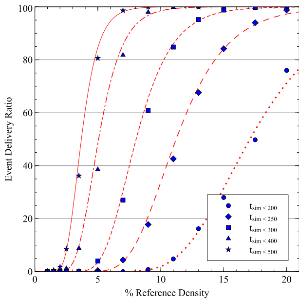
(c) Delivery Ratio of Wiener Mobility Model
