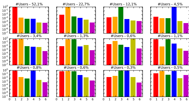
Fig. 7. Cluster of users based on their conversations on Twitter using K-Means and their relative size. We chose k = 12 clusters based on the silhouette coefficient, average cluster size and inertia which were 0.953, 31697.42 and 2512.27, respectively. These clusters shows possible classification of users and might be related to different users' roles in the organ donation environment.
