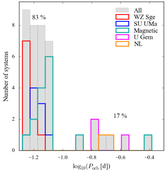
Figure 14. Period distribution for the CVs in the 150 pc sample. The majority of the systems are found below the period and, accounting also for the two WZ Sge-type stars without an orbital period determination, make up for \approx 83 per cent of the observed systems.
