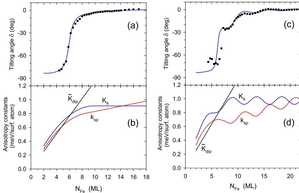
FIG. 6. (a), (c) Experimental values of tilting angle \delta (squares) as a function of the thickness of Fe films on Ag(116) and the theoretical dependence \delta vs N_{\text{Fe}} (solid line) obtained by fitting (b), (d) the model dependencies of the anisotropy constants; (a), (b) T = 300 K and (c), (d) T = 5 K.
