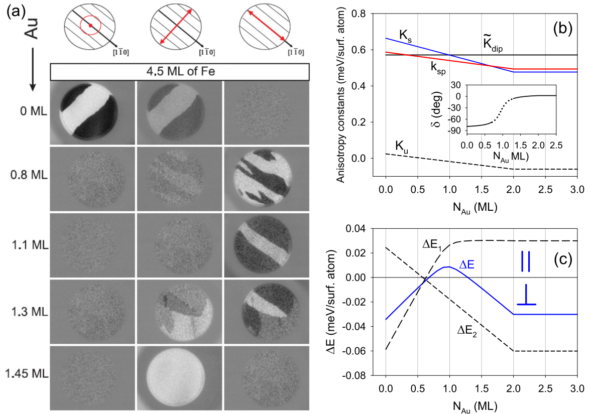
FIG. 10. (a) SPLEEM images with varying thickness of Au film grown on Fe(4.5 ML)/Ag(116) obtained at 130 K. Gray level, with respect to the background corresponding to zero magnetic contrast, represents orientation of magnetization with regard to the polarization of the incident electron beam (light and dark areas correspond to parallel and antiparallel orientations, respectively). Polarization direction of the incident beam is indicated on the top of the image columns. The images are 11.5 \mu\text{m} in diameter; (b) the anisotropy constants (fitted as described in text); (c) the energy difference \Delta E = E_{\perp}^{(\text{min})} - E_{\parallel} (and its components \Delta E_1 = (1/2)(K_{\text{dip}} - K_s - K_{\text{eff},\perp}) and \Delta E_2 = K_u ) between the states with magnetization perpendicular and parallel to the steps. The tilting angle [inset in (b)] is found for the orientation perpendicular to the steps (spontaneous or forced within the model) and marked with the solid line if \Delta E < 0 and with the dotted line if \Delta E > 0 .
