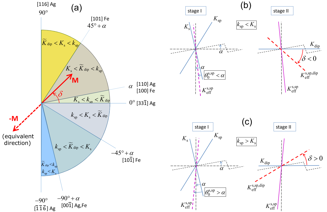
FIG. 3. (a) Tilting angle versus magnetic anisotropy constants. (b), (c) Superposition of three uniaxial anisotropies within the plane perpendicular to the steps, carried out in two stages. The effective anisotropy K_{eff}^{s,sp} is obtained by superposing the magnetocrystalline anisotropies K_s and K_{sp} in stage I and subsequently added to the shape anisotropy K_{dip} in stage II, resulting in the final effective uniaxial anisotropy K_{eff}^{s,sp,dip} = K_{eff,\perp} . The superposition is done in the two cases: (b) k_{sp} < K_s and (c) k_{sp} > K_s .
