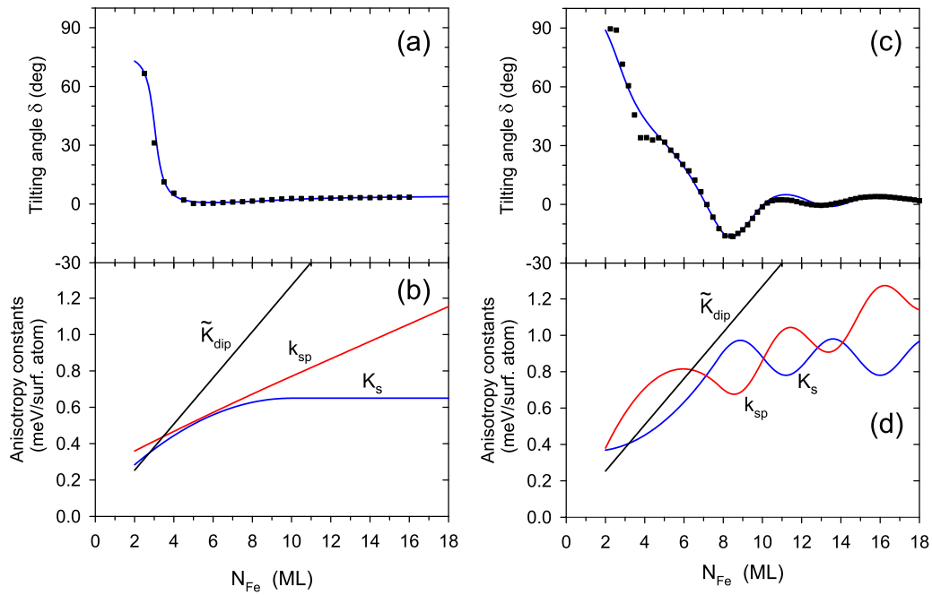
FIG. 7. (a), (c) Experimental values of tilting angle \delta (squares) as a function of the thickness of Au(15 ML)-covered Fe films on Ag(116) and the theoretical dependence \delta vs N_{\text{Fe}} (solid line) obtained by fitting (b), (d) the model dependencies of the anisotropy constants; (a), (b) T = 300 K and (c), (d) T = 5 K.
