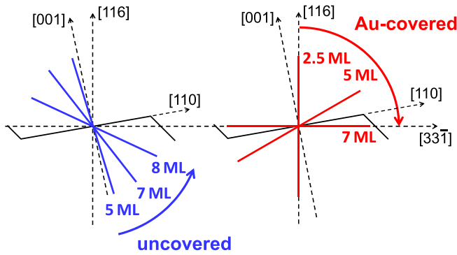
FIG. 8. Schematic of the magnetization easy-axis rotation for uncovered and Au-covered Fe/Ag(116) films upon increasing the Fe film thickness, as obtained from MOKE measurements of the tilting angle at 5 K.
