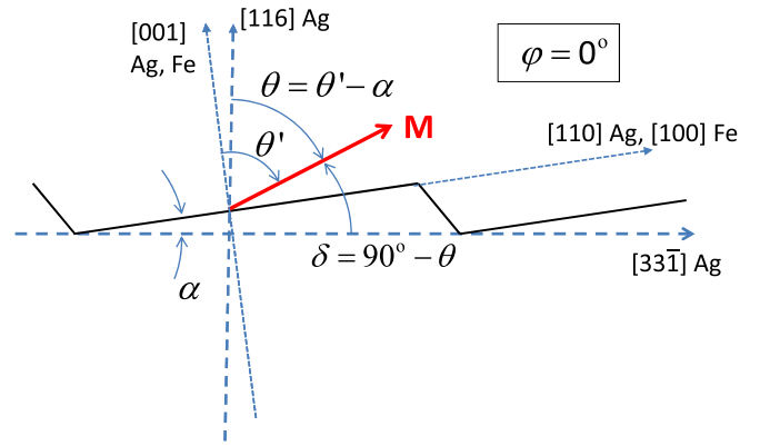
FIG. 2. Magnetization orientation characterized (equivalently) by the angles \delta , \theta , and \theta' within the plane perpendicular to the steps for a Fe film on the Ag(116) surface with the vicinal angle \alpha = 13.3^\circ .
