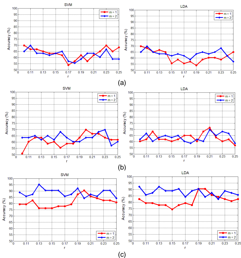
Figure 2. Classification Results with Tuning Parameters of m = 1-2 and r = 0.10 - 0.25 on MSE Method with Feature Vectors Input: (a) SpO2, (b) PR, and (c) SpO2-PR Signals
