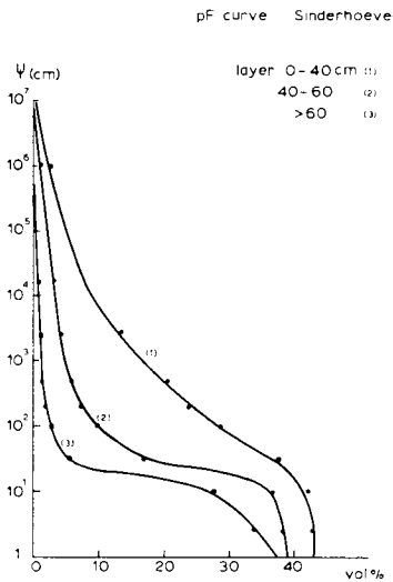
Fig. 1 Soil moisture characteristics.
