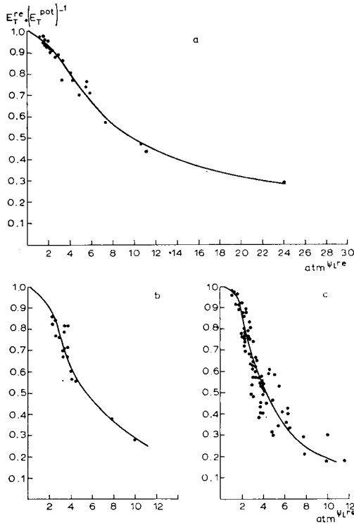
Fig. 9 The relation between the ratio E_T^{re}/E_T^{pot} and the real suction in the leaves ( \psi_l^{re} ) for 3 groups of soil cover. a. soil cover < 50 %; b. soil cover between 50 and 80 %; c. soil cover > 80 %
