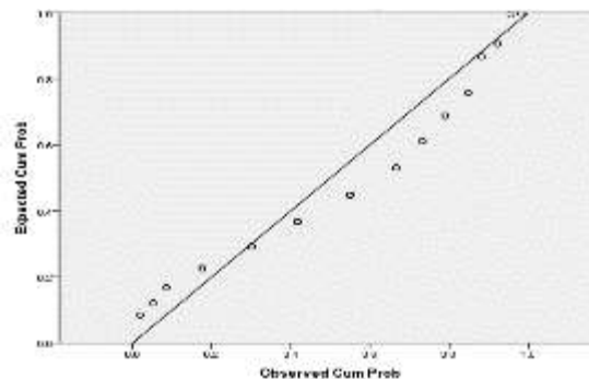
Gambar 1. Normal P-P Plot of Model Pembelajaran
