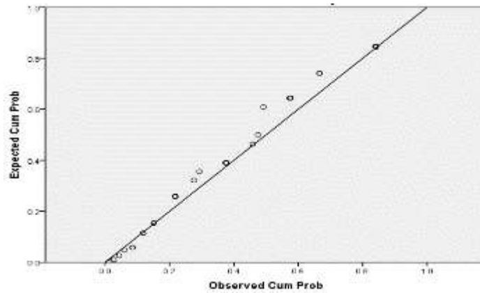
Gambar 2. Normal P-P Plot of Motivasi Belajar Siswa
