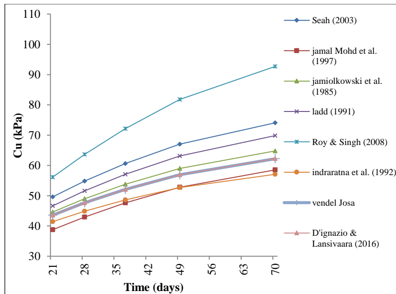
Figure 4. Comparison of Cu curves for normally consolidated mucky soil, R2288
