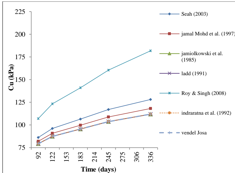
Figure 3. Comparison of Cu curves for over consolidated clay, R3058
