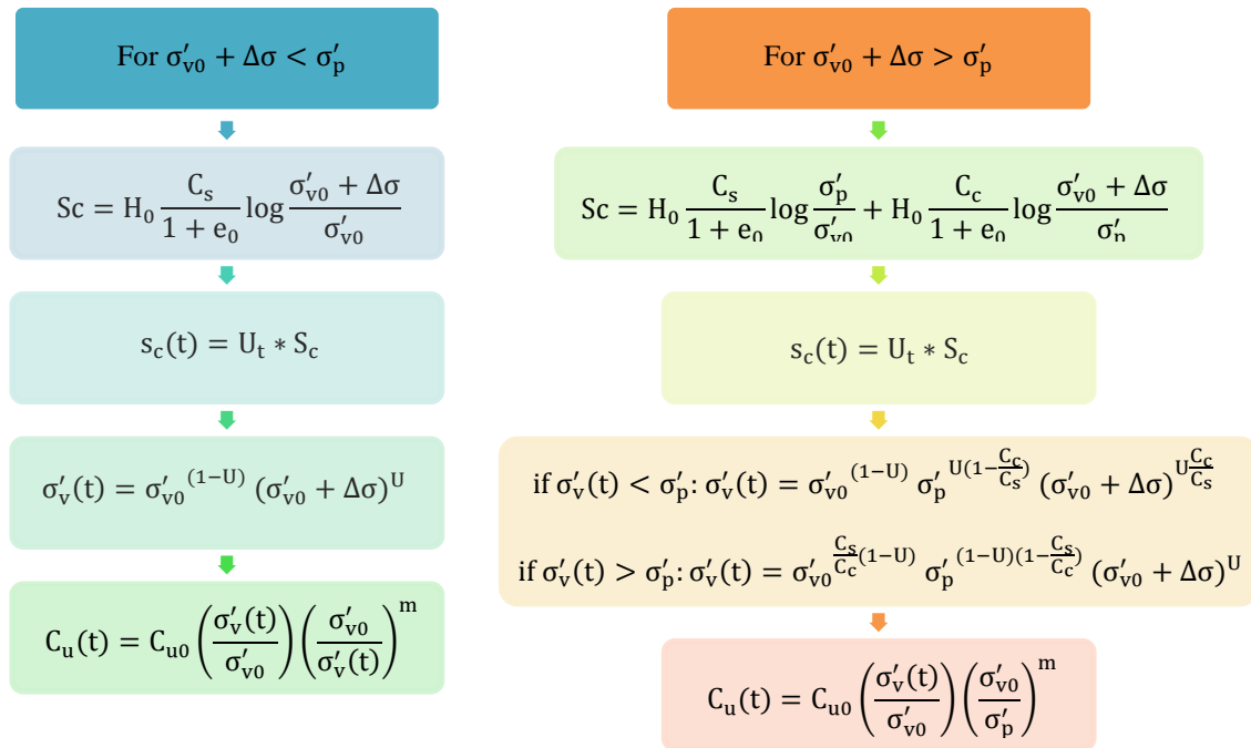
Figure 1. Proposed method for obtaining the increase in shear strength
