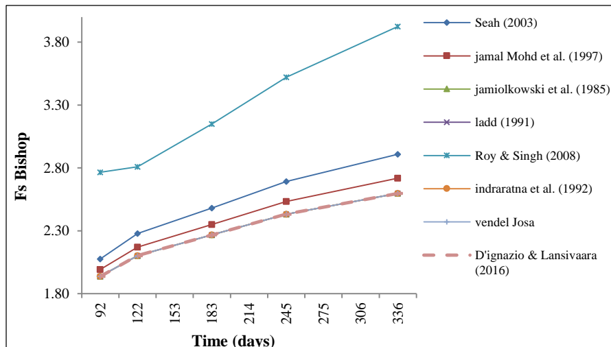
Figure 6. Variation of factor of safety with time R3058
