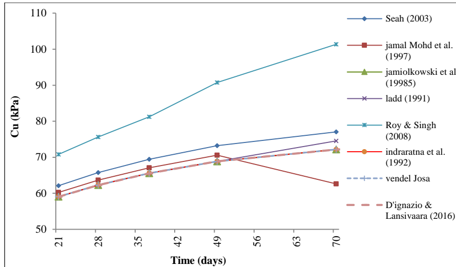
Figure 5. Comparison of C_u curves for over consolidated silty clay that becomes normally consolidated after loading, R2288
