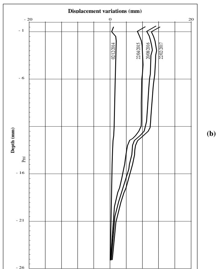
Figure 9. (a) Lateral displacements at various time periods R3089, PR308+830; (b) Lateral displacements at various time periods R3089, PR308+920
