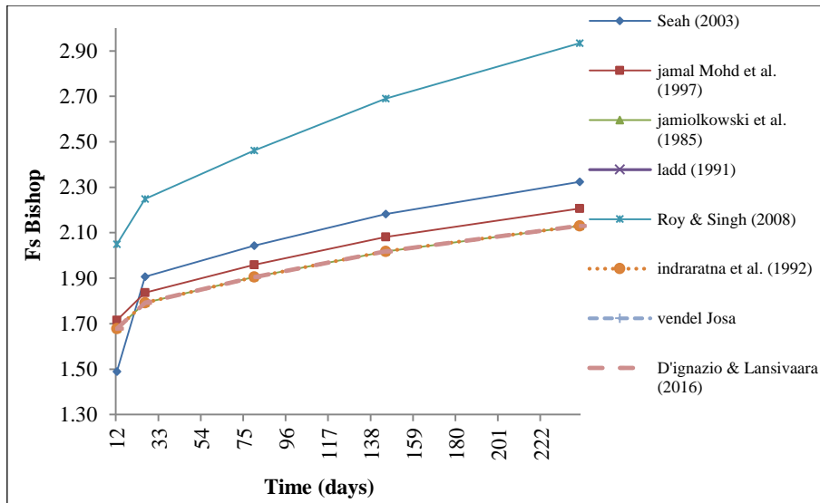
Figure 7. Variation of factor of safety with time R3089
