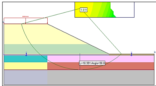
Figure 8. Critical slip surface after 12 days of construction R3089
