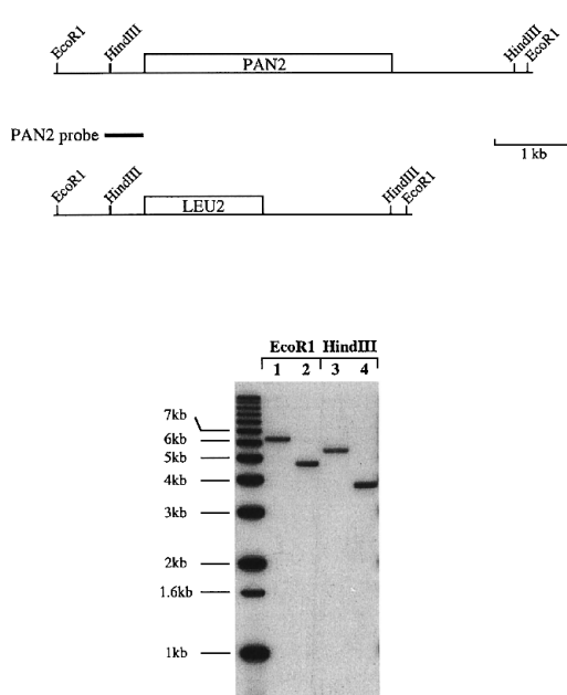
Fig. 5. Southern blot for PAN2 confirms disruption of the PAN2 gene in strain YAS1837. A 450-nucleotide radioactive PAN2 probe was hybridized to a Southern blot containing yeast genomic DNA digested with the indicated enzymes. Lanes 1 and 3, wild type strain (YAS306); lanes 2 and 4, PAN2 deleted strain (YAS1837). Molecular size markers (kb) are indicated. The diagram indicates the relative positions of the restriction sites, the placement of the LEU2 marker in the PAN2 gene, as well as the position of the PAN2 probe.
