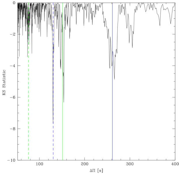
Figure 3. Output of the KS test indicating the spacing for the period sequences. The solid blue (green) line indicates the period spacing for the \ell = 1 (2) sequence with the dashed line being the overtone alias.
