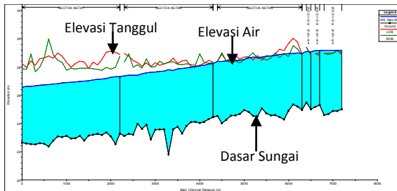
Gambar 8. Hasil Model Unsteady flow
