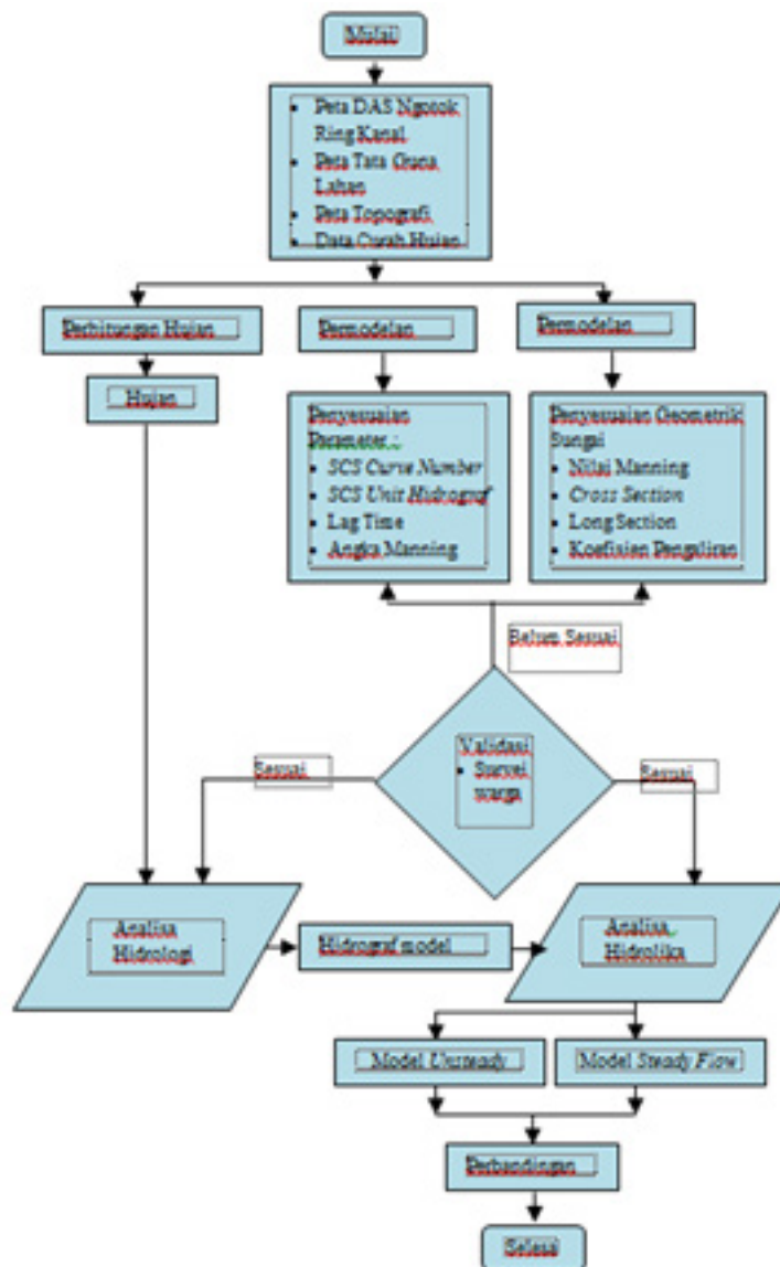
Gambar 3. Diagram Alir Penelitian
