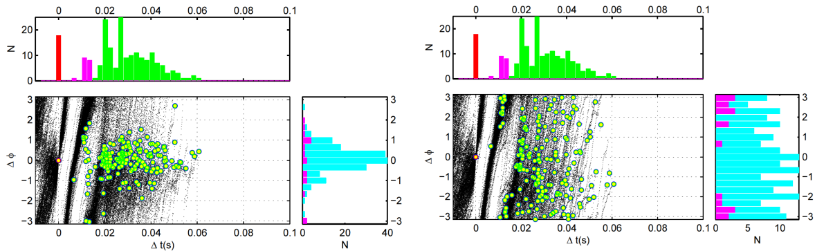
Fig 3: Left set of panels: ELM occurrence times and VLD3 phase difference between all pairs of ELMs in the flat-top of JET plasma 83769. Right set of panels: same format as left panel, but with randomly shuffled time order of the inter-ELM time intervals. Each set of panels is as follows. Main panel: VLD3 instantaneous phase, modulo 2\pi , plotted as a function of time, up to the occurrence time of the next ELM. The coordinates are time, and phase difference from the occurrence time of the first ELM. ELM occurrence times are marked on each VLD3 trace with yellow filled red circles (first ELM) and green circles (second ELM). Right hand panel: histogram of VLD3 phase difference at the time of the second ELMs, for inter-ELM time intervals \Delta t < 0.015 (magenta) and for all ELMs (cyan). Top Panel: histogram of inter-ELM time intervals.
