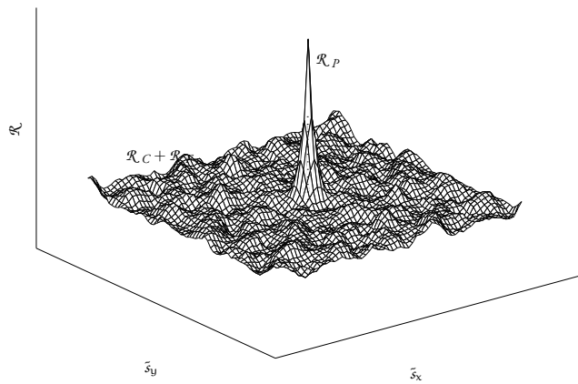
Figure 3.9: Typical correlation plane for single-frame single-exposure mode.
