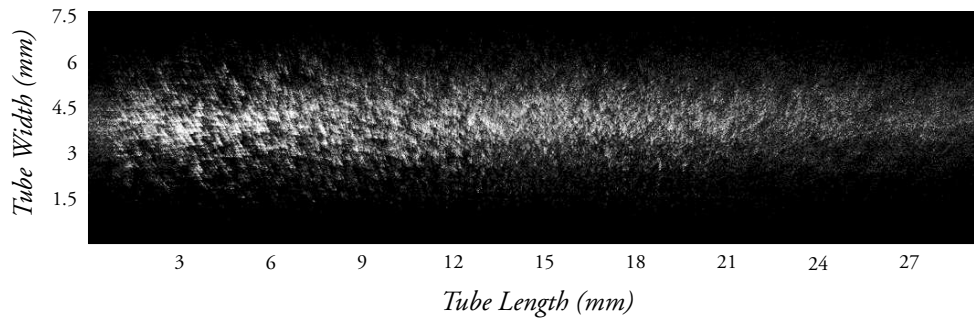
Figure 6.14: The illumination profile as recorded by the CCD camera with an illumination duration of 0.1 ms.
