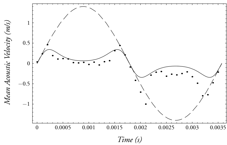
Figure 6.22: Comparison between CBC-processed experimental acoustic velocities (•), the theoretical fit considering the out-of-plane effect (—) and the expected values (---) for the first mode of the tube with SPL = 151.2 dB and \tau_i = 0.2 ms. The fitted curve corresponds to a Gaussian light sheet with a thickness of 0.05 mm and a deviation angle of 9^\circ .
