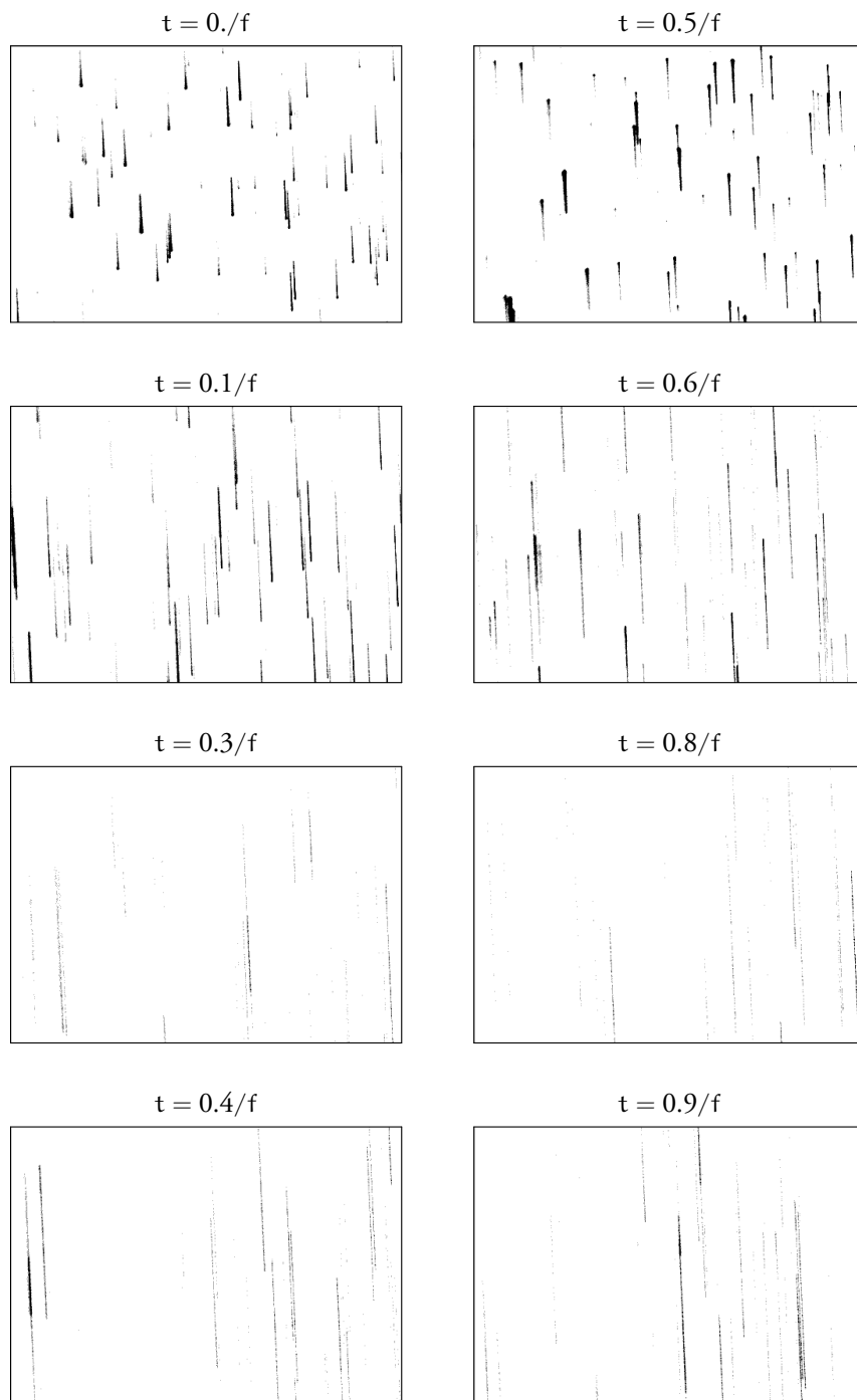
108 Figure 6.16: Visualisation of sound field in the non-anomalous location of the tube.
