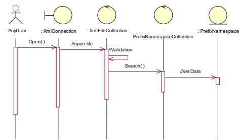
Gambar 13. Sequence diagram open file
