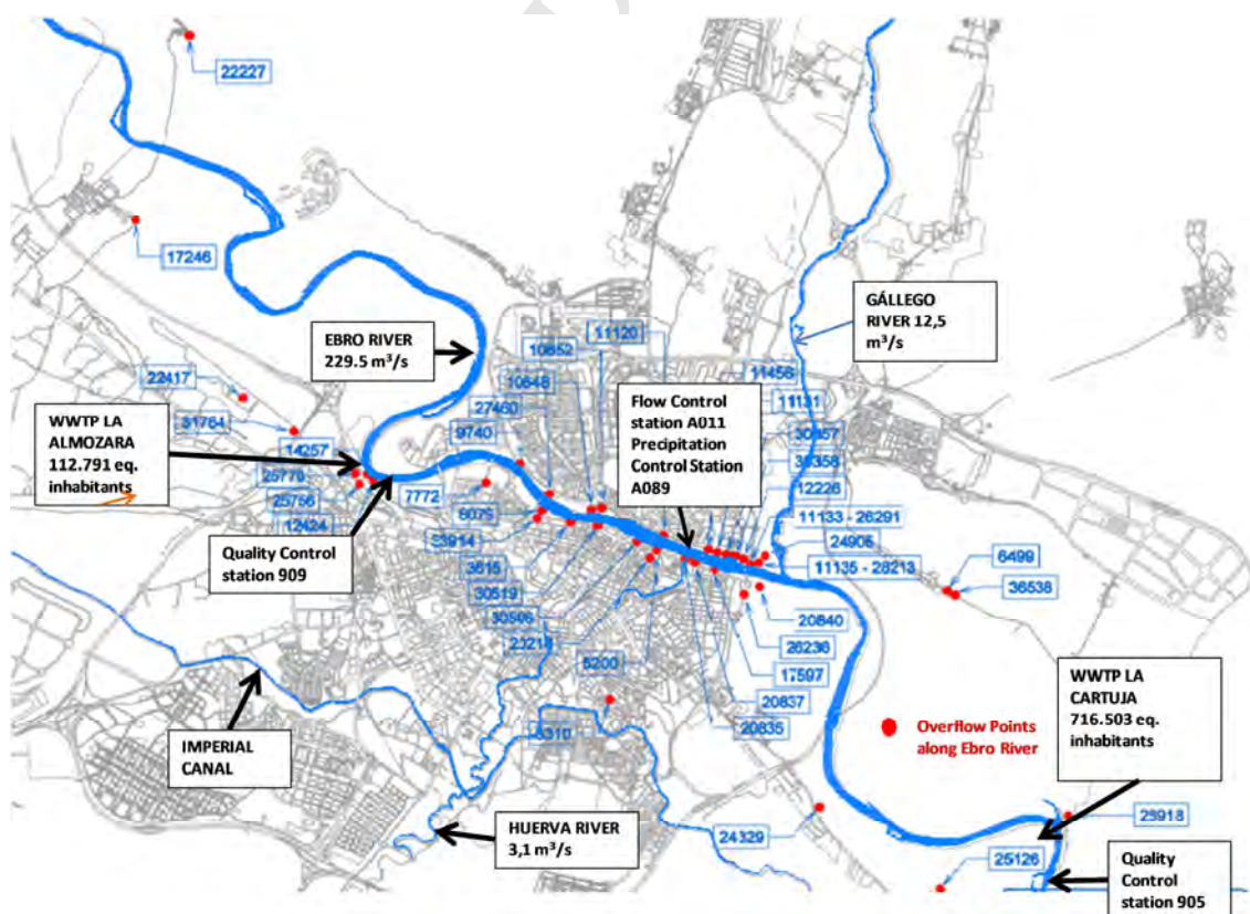
Figure 1. Natural and artificial drainage networks of Zaragoza
