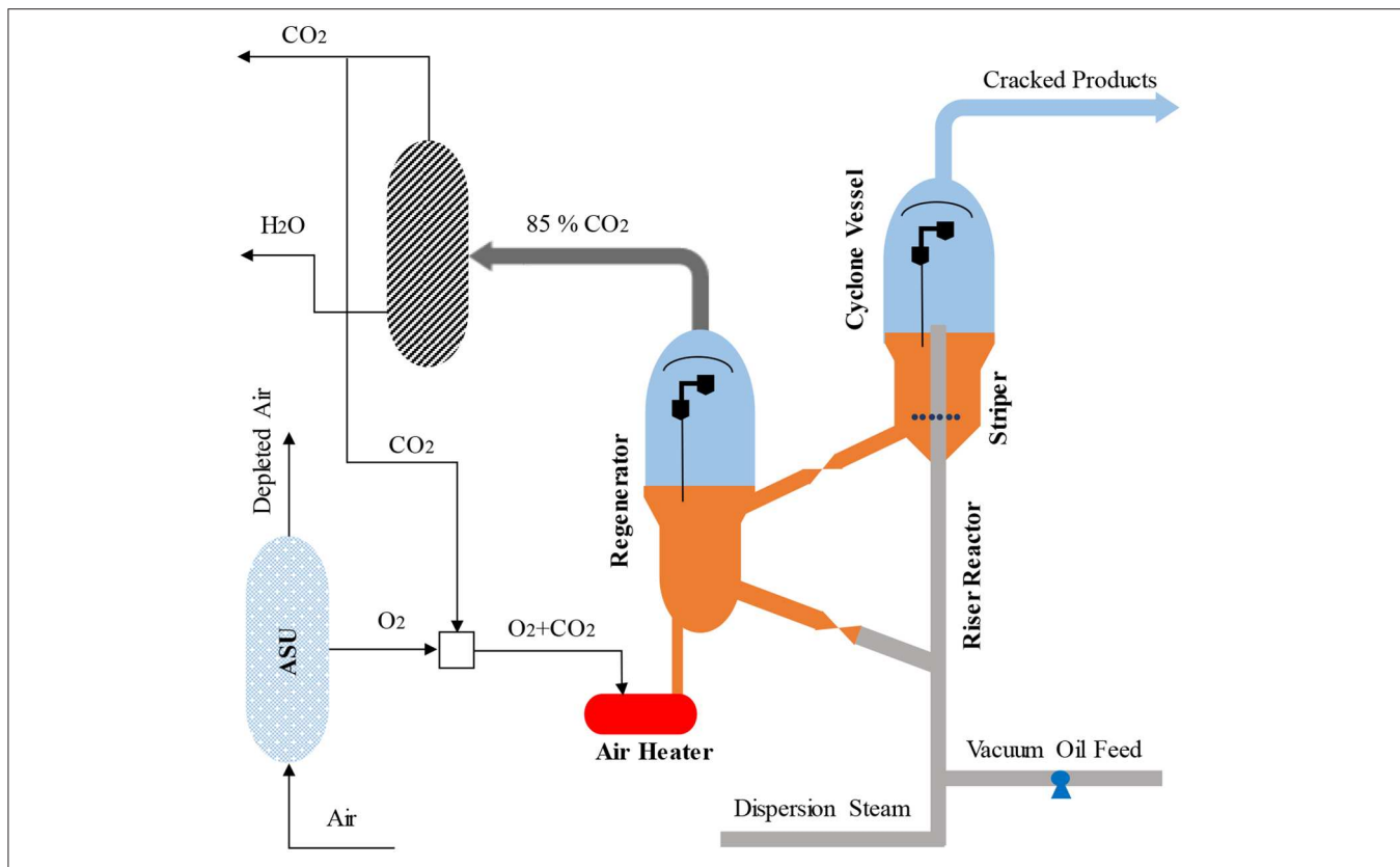
FIGURE 7 | Oxy-combustion capture in FCC units adapted from Miracca and Butler (2015) with permission from BP Group Technology.
