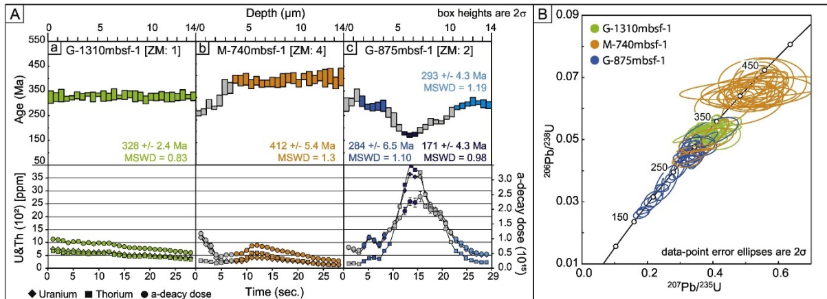
Fig. 3. U-Pb depth profiling: (A) U-Pb depth profiling including the calculated 206 Pb/ 238 U weighted mean ages for the respective zircon crystal (upper panels) (Individual boxes represent one-second increments within a single analysis, 2-sigma) vs. U and Th [ppm] concentrations as well as α-decay [α/mg] damage accumulation (lower panels). Three main patterns are observed: (A.a.) Relatively “closed system”; (A.b.) Younger rim and older interior ages; and (A.c.) Older rims and younger interior zones. The age spectra display 206 Pb/ 238 U age domains and U and Th [ppm] versus depth after downhole and mass fractionation correction. (ZM = zircon morphology). Pit ablation depth estimated based on previous laboratory calibration measurements using a Bruker Optical Profilometer. (B) Wetherill Concordia plot (1956) for each individual, complete, analyses (30/40 s). (Tera Wasserburg diagrams are visualized in Fig. S3).
