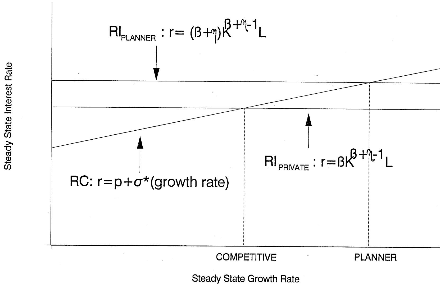
FIGURE 4: ARROW-SHESHINSKI-ROMER MODEL
