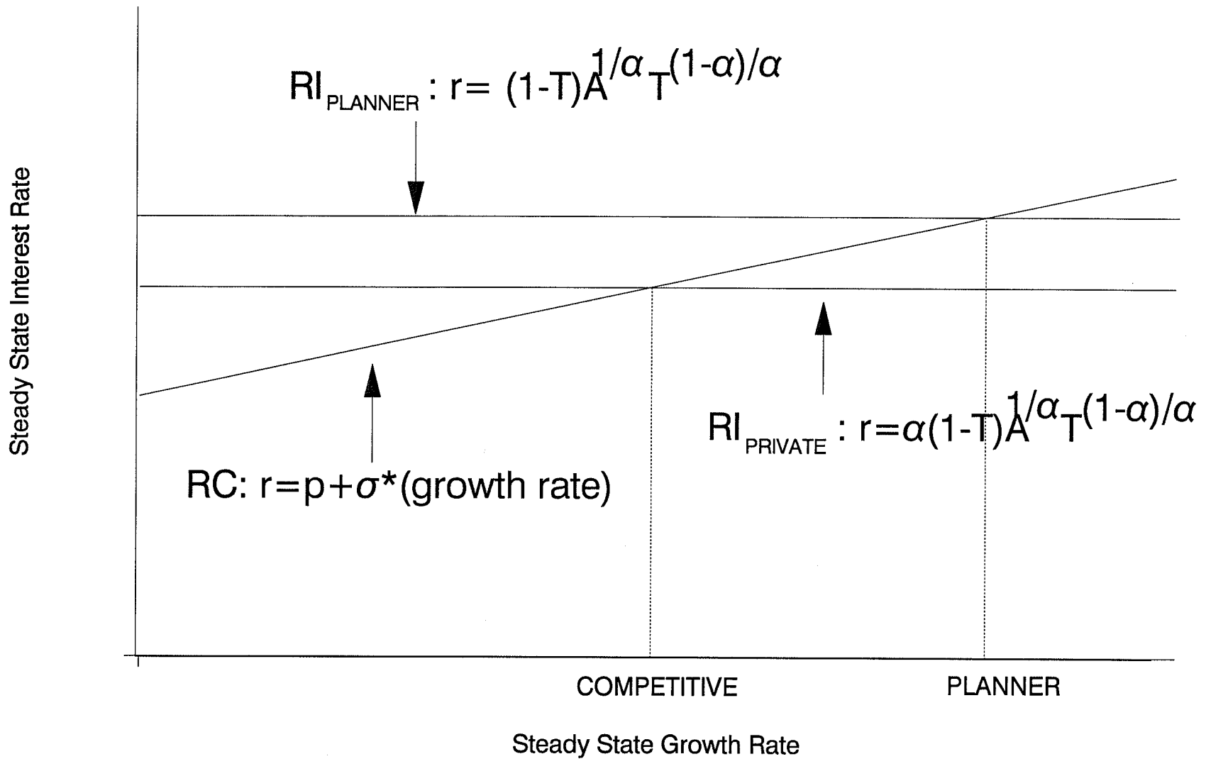
FIGURE 3: BARRO MODEL
