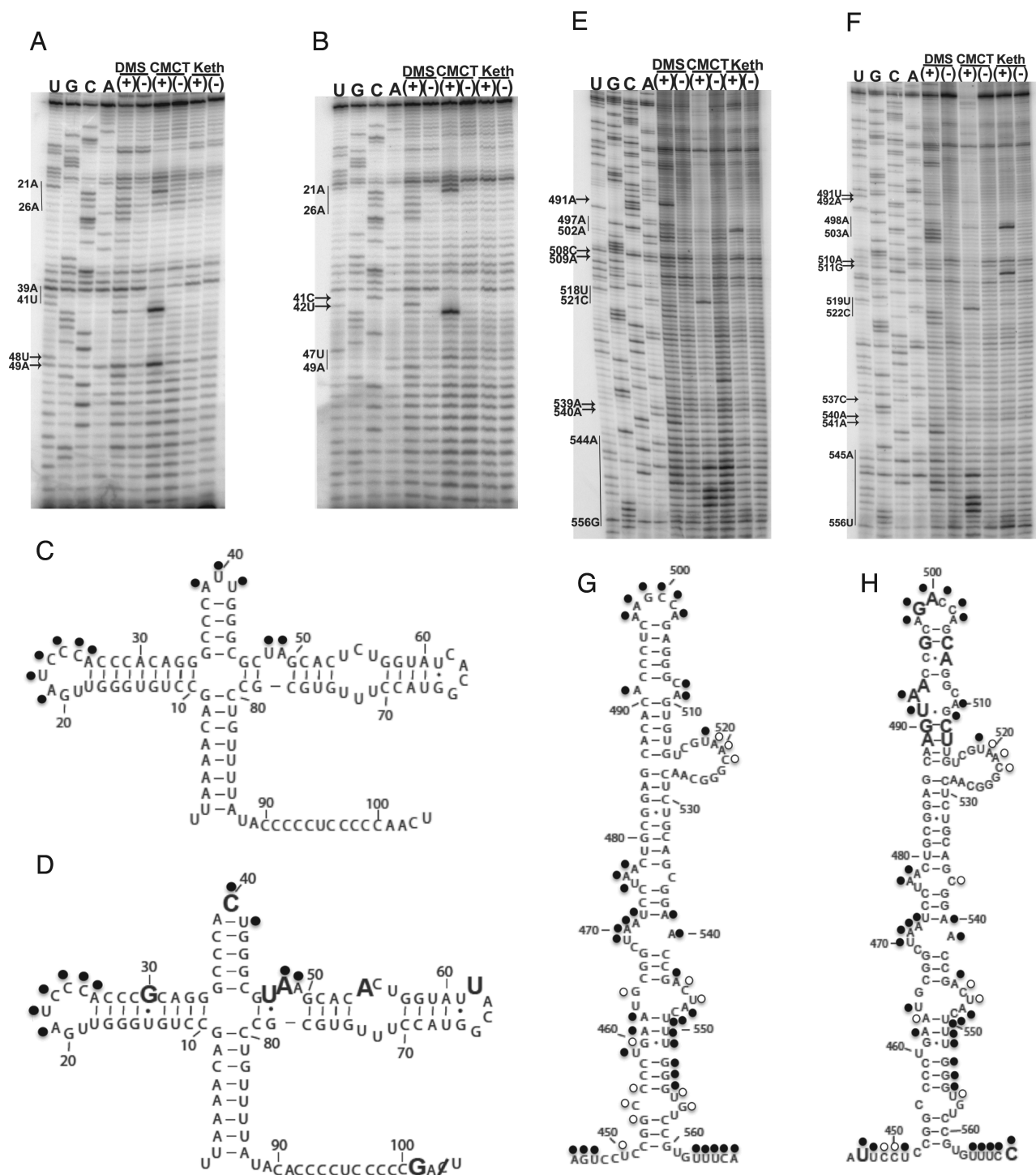
Figure 5. Chemical probing results for CV-B3/28 and CV-B3/GA domains I and V. For all sequencing gels, arrows indicate modified positions and vertical lines between two nucleotide positions indicate that all positions between and including the positions shown are modified. Sequencing tracks indicating the nucleotide positions are labelled A, C, G and U. Tracks with chemically modified RNA are labelled (+) and tracks with unmodified RNA are labelled (-). (A) 12% sequencing gel showing CV-B3/28 domain I. (B) 12% sequencing gel showing CV-B3/GA domain I. (C) Predicted secondary structure model of CV-B3/28 domain I. Modified positions are indicated with a circle. Closed circles indicate heavily modified positions and open circles indicate moderately modified positions. (D) Predicted secondary structure model of CV-B3/GA. Modified positions are indicated with a circle. Closed circles indicate heavily modified positions and open circles indicate moderately modified positions. Enlarged nucleotide positions are substituted or inserted in CV-B3/GA. The position with the slash is deleted in CV-B3/GA. (E) 12% sequencing gel showing CV-B3/28 domain V. (F) 12% sequencing gel showing CV-B3/GA domain V. (G) Predicted secondary structure model of CV-B3/28 domain V. Modified positions are indicated with a circle. Closed circles indicate heavily modified positions and open circles indicate moderately modified positions. (H) Predicted secondary structure model of CV-B3/GA domain V. Modified positions are indicated with a circle. Closed circles indicate heavily modified positions and open circles indicate moderately modified positions. Enlarged nucleotide positions are substituted in CV-B3/GA.
