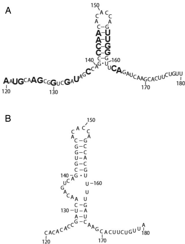
Figure 6. Models for structurally distinct domain II folding in CV-B3/GA and CV-B3/28. (A) CV-B3/GA. (B) CV-B3/28. The enlarged nucleotide positions are substituted or inserted in CV-B3/GA.
