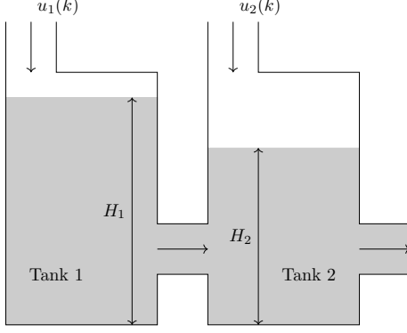
Figure 2. Plant scheme.
