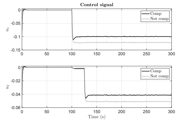
Figure 9. Comparison between control signal with and without compensation for the case without fault signal.
