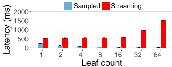
Figure 7: Scalability of vizketches as we add more leafs and shards together. Ideal scalability would be constant latency.
