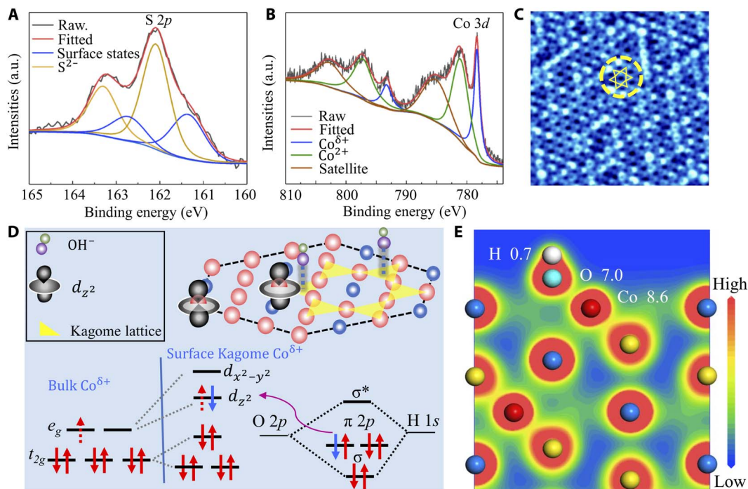
Fig. 4. Surface structure and OER mechanism. (A) Detailed XPS analysis of the prepared single crystal. High-resolution XPS spectra for (A) S\ 2p and (B) \text{Co}\ 3d . (C) STM topography of a cleaved \text{Co}_3\text{Sn}_2\text{S}_2 single-crystal thin flake showing an area of 8 nm by 8 nm. The Kagome lattice is highlighted by yellow lines in the circle. (D) Schematic representation of the favored OH uptake with the Co 3d orbitals. The exfoliation between the S—Sn plane breaks the octahedral symmetry of the surface Co atoms in the Kagome lattice (highlighted by yellow triangle). The empty 3d_{z^2} orbital points to the p orbital of the OH group, resulting in a strong bonding between them. (E) Contour plots of the total charge distribution of \text{Co}_3\text{Sn}_2\text{S}_2 single crystal with one OH group bonded to the Co atoms. Electronic charges are distributed in the vicinity of Sn atoms. However, for Co atoms, one can see the electron transfer through the Co—O bonding. a.u., arbitrary units.
