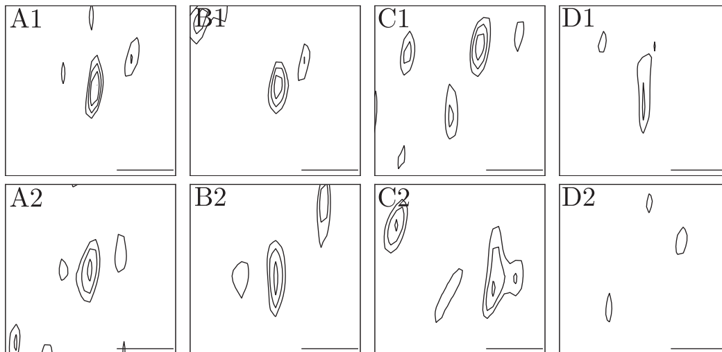
Figure 2. Maps of the lensed components of HS 0810+2554 made using three different weighting schemes, from a natural weighting scheme (top) to a compromise weighting scheme between natural and uniform (bottom), with robustness parameters of 5, 1, and 0 in the Briggs' weighting scheme, respectively. In all images contours have been drawn at (-3, 3, 4, 5, 6) \times 7.2 \mu\text{Jy} and the scalebar represents a length of 10 mas.
