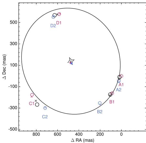
Figure 8. The best-fitting model of HS 0810+2554 obtained using the positions of components in the EVN image and HST observations as constraints. The lensing galaxy was modelled as an SIE and is centred on the vertical cross. The tangential critical curve is represented by the thin black curve and the caustic by the thick black curve. The predicted positions (crosses) of lensed components are plotted for comparison with observed component positions (open circles). The predicted positions of the components in the source plane (filled circles) are also plotted. Source 1 is represented by red markers, source 2 by blue, and the source observed by HST in black. Model parameters and uncertainties are reported in Table 3 and derived parameters in Table 4. Model and observed component positions are reported in Table 5. All positions are plotted with respect to component A1.
