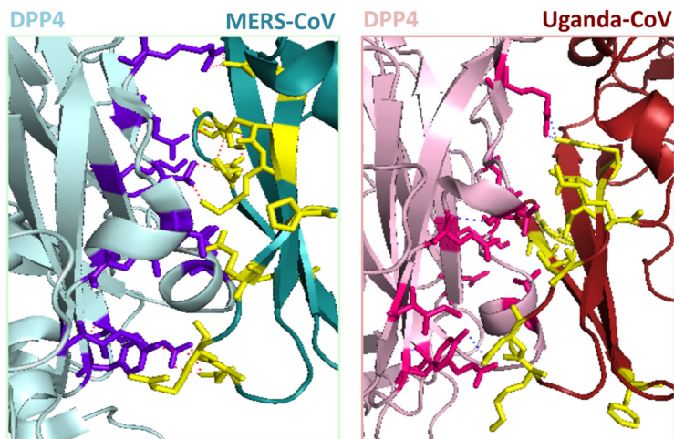
FIG 3 The spike protein of PREDICT/PDF-2180 is highly divergent. (A) A nucleotide identity Simplot shows that PREDICT/PDF-2180 and NeoCoV are closely related to MERS-CoV across much of the genome but are highly divergent in subunit 1 of the spike protein, suggesting that they may have different receptor binding properties. (B) Variation in key amino acid binding residues (*) and modeling to human DPP4 both suggest that PREDICT/PDF-2180 is unable to bind to DPP4.
