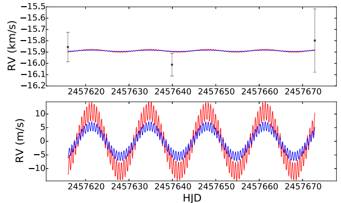
Figure 4. Recon spectra of EPIC 220674823 show no stellar RV signal within errors (rms = 110 m s ^{-1} ). The combined estimated RV signal of the two planets is plotted for reference (assuming masses of 4.5 and 41 M_{\oplus} in blue and 2.3 and 20.5 M_{\oplus} in red). The bottom panel shows a zoomed-in version of the estimated signal, which, with an estimated amplitude of 2–11 m s ^{-1} , is easily accessible by more precise RV instruments.
