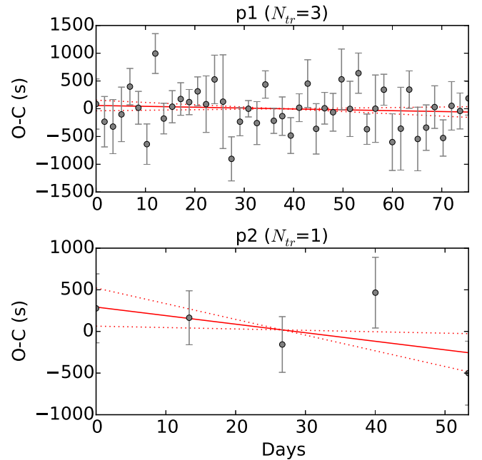
Figure 3. Observed minus calculated mid-transit times for p1 (top) and p2 (bottom). For p1, which does not have sufficient precision to individually fit each transit, we stacked N_{tr} = 3 consecutive transits together, for one point every 1.7 days; the pattern is similar if more consecutive transits were stacked instead. For p2, each individual transit was fit.
