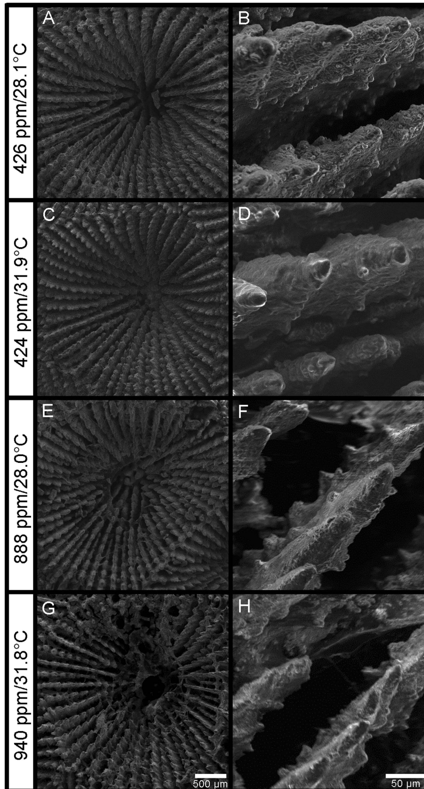
Figure 4. Secondary electron images of S. siderea corallites (left column) and septae (right column) produced under p\text{CO}_2 -temperature treatments of 426 ppm- v/28.1^\circ\text{C} (A,B), 424 ppm- v/31.9^\circ\text{C} (C,D), 888 ppm- v/28.0^\circ\text{C} (E,F), and 940 ppm- v/31.8^\circ\text{C} (G,H). Corallites are less infilled owing to thinner septae under conditions of elevated p\text{CO}_2 . Secondary electron images of the coral septae (right column) also reveal that elevated p\text{CO}_2 decreases septal rugosity, apparently by reducing the prominence of the corals' aragonite nucleation sites, their so-called centers-of-calcification.
