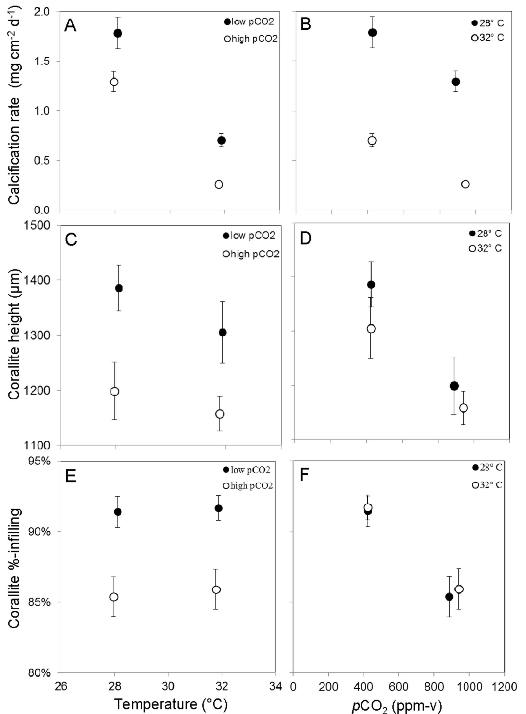
Figure 1. Effect of temperature and p\text{CO}_2 on average calcification rates (A,B), corallite heights (C,D), and %-corallite in-filling (E,F) of S. siderea corals reared in the four crossed temperature- p\text{CO}_2 treatments (426 ppm-v/28.1°C; 424 ppm-v/31.9°C; 888 ppm-v/28.0°C; 940 ppm-v/31.8°C). Mixed effects modelling reveals that both p\text{CO}_2 and temperature are significant predictors of coral calcification rate, while p\text{CO}_2 alone is a significant predictor of corallite height and %-infilling, across the 60-day experiment. Bars show standard error.
