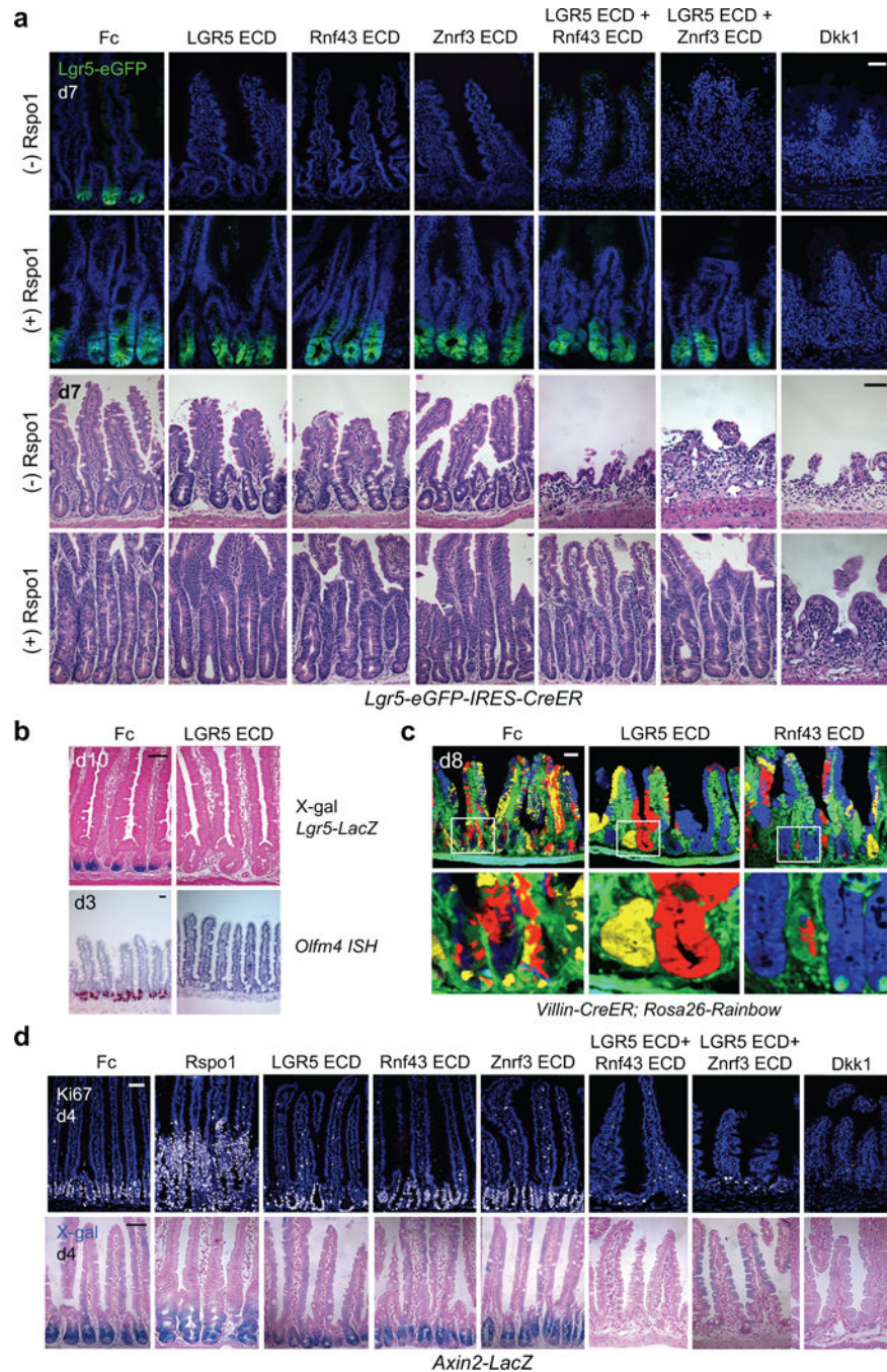
Figure 1. Pan-Rspo inhibition by systemic overexpression of LGR5, Rnf43 or Znr3 ECDs
