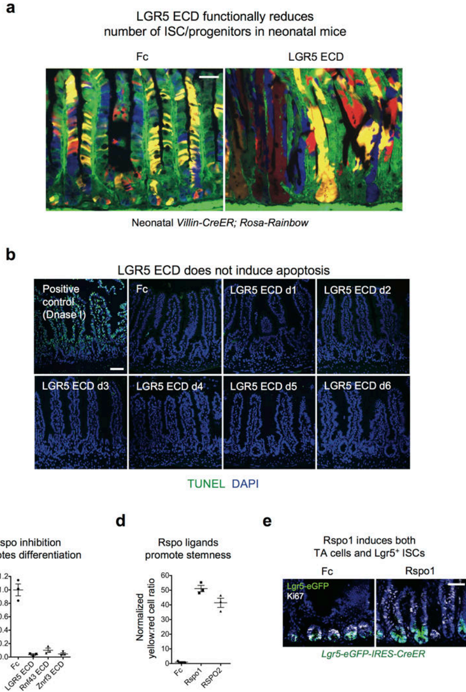
Extended Data Fig. 3. LGR5 ECD reduces ISC/progenitors but not via apoptosis a , LGR5 ECD functionally reduces number of ISC/progenitors in neonatal mice. Multi-color clonal labeling of intestinal epithelial cells in jejunum of neonatal Villin-CreER ; Rosa26 -
