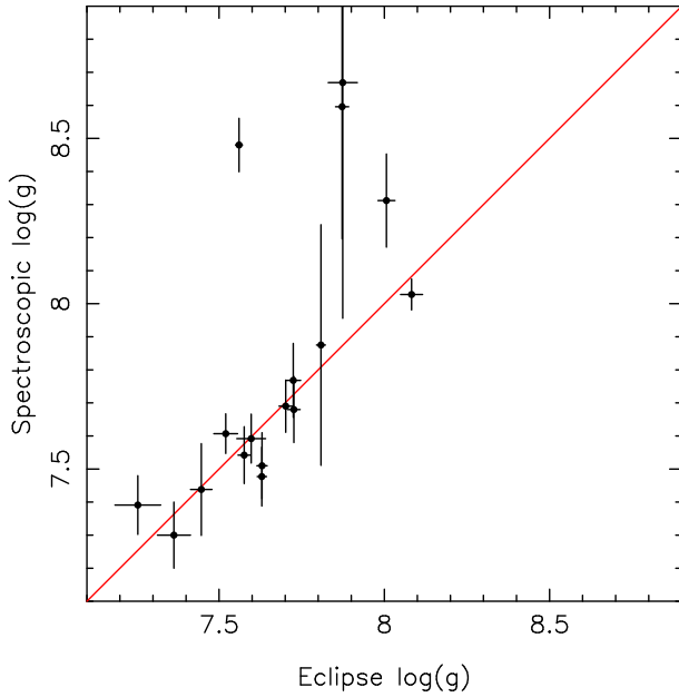
Figure 13. Comparison between the surface gravities determined from the model atmosphere fits to the X-Shooter spectroscopy, and those computed from the mass and radius values measured from the light curves.
