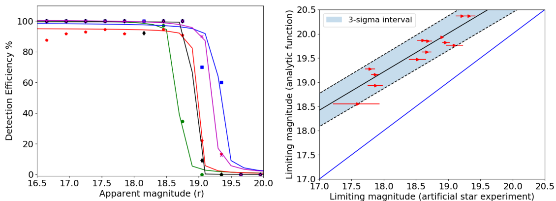
Fig. 2.— Left panel: Transient detection efficiency as a function of apparent magnitude for 5 DLT40 fields. The lines are the best fit to the curve. The limiting magnitude is chosen at 50% efficiency. Right panel: We compare the limiting magnitude computed for each image using its zeropoint and an analytical function with the limiting magnitude computed with artificial star experiments on difference images. This linear relation has been used to scale the limiting magnitude computed for each frame (given its zeropoint) to a more realistic limiting magnitude estimate for SN and/or kilonova detection.
