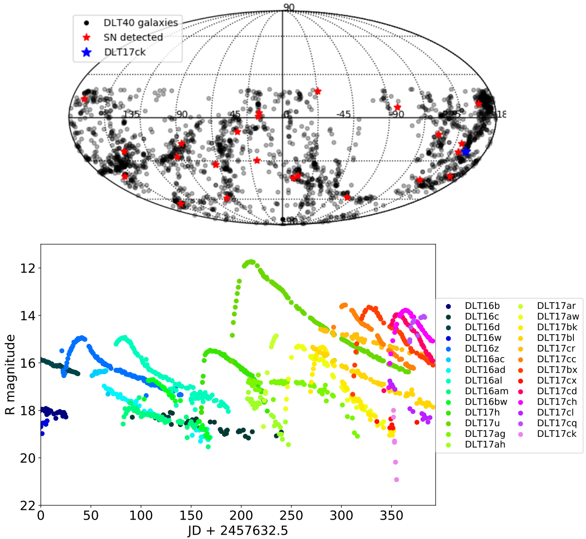
Fig. 1.— Top panel: The DLT40 galaxy catalog (black points). The SNe discovered during the first year of DLT40 are also shown (red points) together with the kilonova DLT17ck (blue point). Lower panel: DLT40 light curves of all the SNe (and the kilonova) discovered during the first year of the search.
