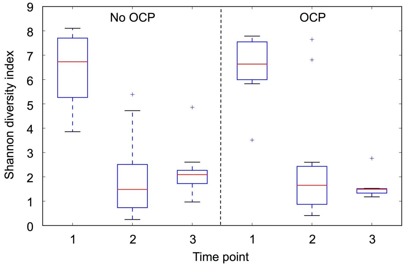
Figure 2. The impact of oral colostrum priming on diversity of the oral microbiota Shannon diversity index by group and time point. OCP-oral colostrum priming. Time points: 1 (1–2 days of life), 2 (8–9 days of life), 3 (30 days of life). Box represents 25 th and 75 th percentiles, line represents median, whiskers represent maximum and minimum, and plus signs represent outliers.
