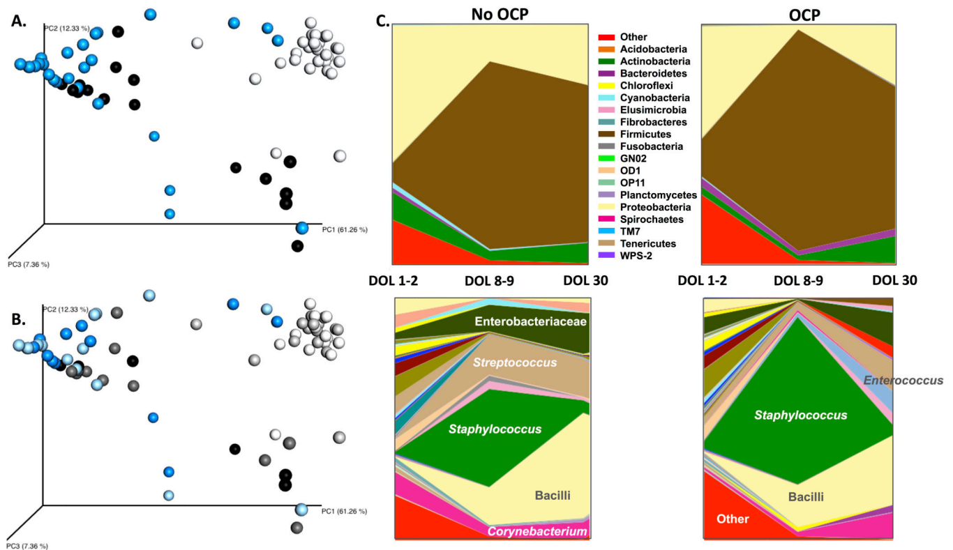
Figure 3. Unweighted unifrac principal coordinate analysis (PCoA) of oral microbiota by time point and time point/ treatment group
