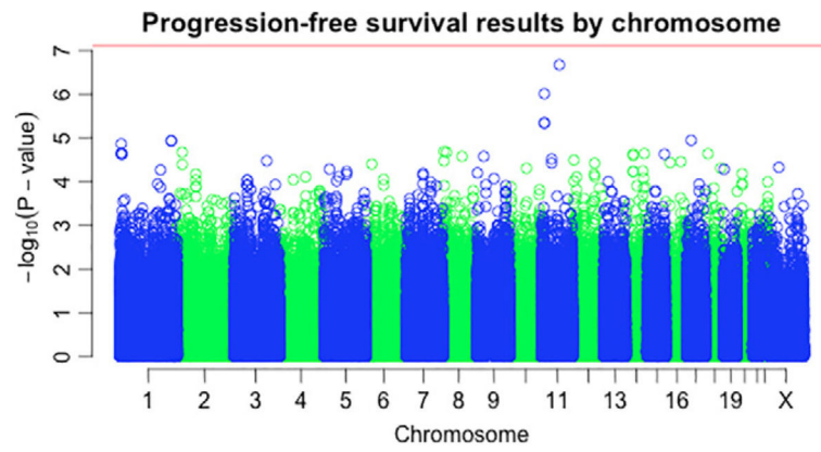
Fig. 2. Manhattan plot for progression free survival. The horizontal red line displays the Bonferroni threshold which was not crossed by any polymorphism indicating lack of statistical significance.
