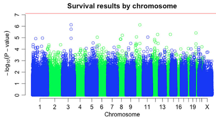
Fig. 1. Manhattan plot for overall survival. The horizontal red line displays the Bonferroni threshold which was not crossed by any polymorphism indicating lack of statistical significance.
