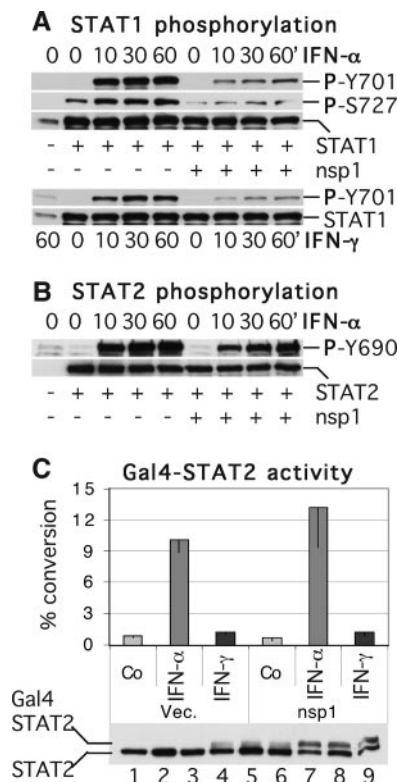
FIG. 5. (A) 293T cells transfected with empty vector (-) or vectors for expression of nsp1 and/or STAT1 \alpha were treated with 2,000 U/ml of IFN- \alpha or IFN- \gamma for 0, 10, 30, and 60 min, and extracts were analyzed by immunoblotting. (B) 293T cells transfected with empty vector (-) or vectors for nsp1 and/or STAT2 were treated with 2,000 U/ml of IFN- \alpha for 0, 10, 30, and 60 min, and extracts were analyzed by immunoblotting. (C) 293T cells transfected with Gal4-STAT2, G5E1bCAT, and empty vector (Vec.) or a vector for nsp1 were left untreated (Co) or treated with 500 U/ml of IFN- \alpha or IFN- \gamma for 18 h, and reporter activity was determined. Extracts were also analyzed by immunoblotting with an anti-STAT2 antibody, which detects the Gal4-STAT2 fusion and endogenous STAT2. Lanes 1 to 3, cells transfected with empty vector; lanes 4 to 6, cells transfected with Gal4-STAT2; lanes 7 to 9, cells transfected with Gal4-STAT2 and nsp1. Cells were left untreated (lanes 1, 4, and 7) or were treated for 18 h with 500 U/ml of IFN- \alpha (lanes 2, 5, and 8) or IFN- \gamma (lanes 3, 6, and 9).
