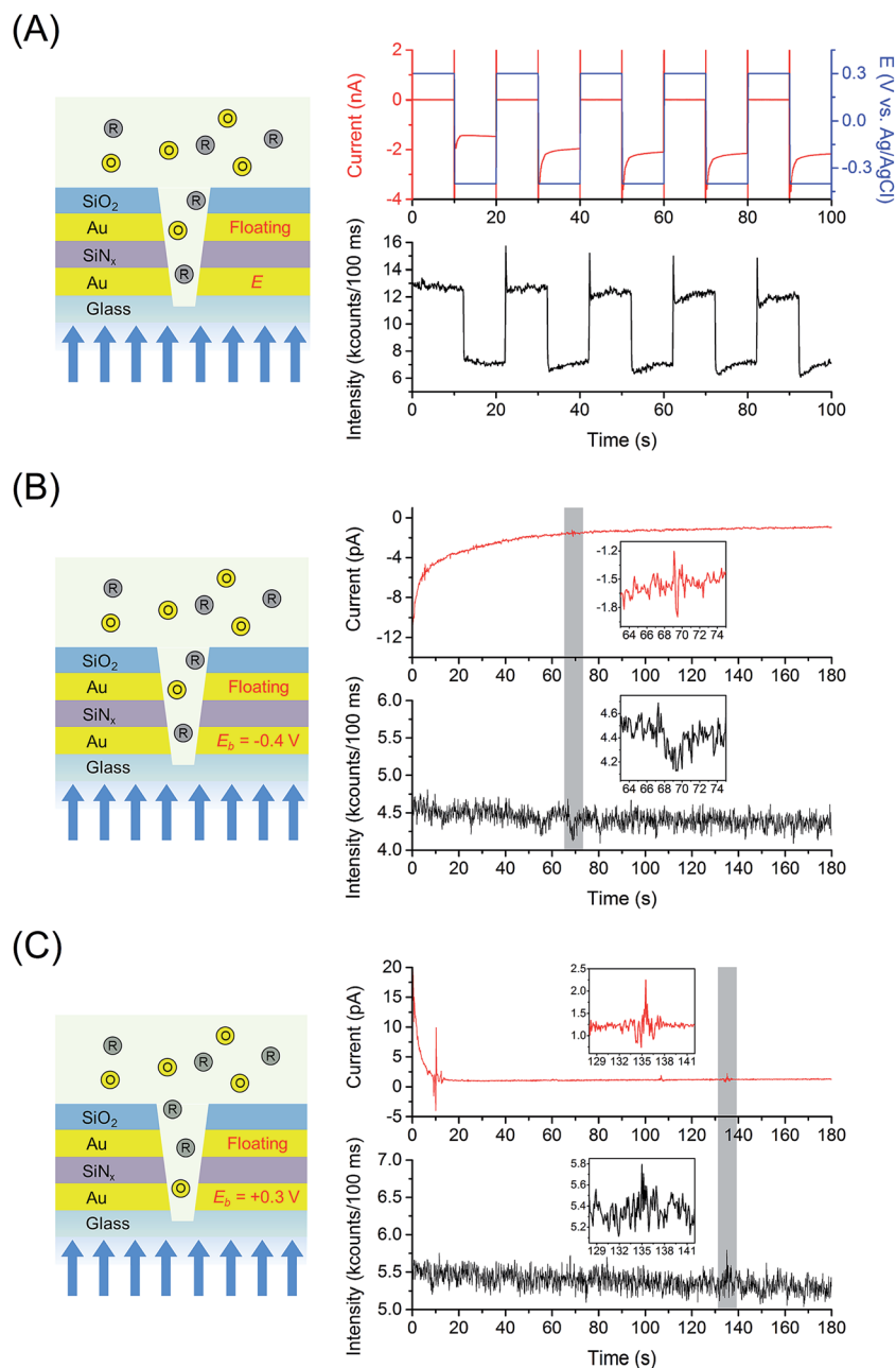
Fig. 3 (A) Experimental scheme and chronoamperometry of 1 \mu\text{M} FMN in 100 mM citrate buffer at pH 2.9. The potential of bottom electrode ( E_b ) is modulated at 10 s intervals between +0.3 V and -0.4 V, while the potential of top electrode ( E_t ) floats. The temporal offset between optical and electrochemical data is caused by a trigger delay between the start of optical vs. electrochemical data acquisition. (B and C) Experimental schemes and current/fluorescence-time traces of 10 nM FMN in 100 mM citrate buffer at pH 2.9. Representative trajectories of the electrical and optical signals are given by the red and black solid lines, respectively. The insets show magnified views of the simultaneous electrical and optical signal excursions, which are highlighted in gray. (B) E_b = -0.4 V vs. Ag/AgCl, while E_t floats. (C) E_b = +0.3 V while E_t floats.
