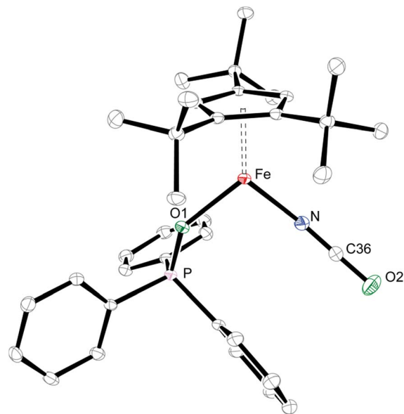
Fig. 4 Thermal ellipsoid plot (30% probability) of the molecular structure of 6 . H-atoms are omitted for clarity. Selected bond distances (Å) and angles (°): Cp' cent –Fe 1.968, Cp' plane –Fe 1.967, Fe–N 1.9530(17), Fe–O1 2.0164(13), O1–P 1.5074(14), N–C36 1.170(3), C36–O2 1.203(6), O1–Fe–N 101.30(7), Fe–O1–P 137.97(8), Fe–N–C36 154.80(18), N–C36–O2 177.2(2).
