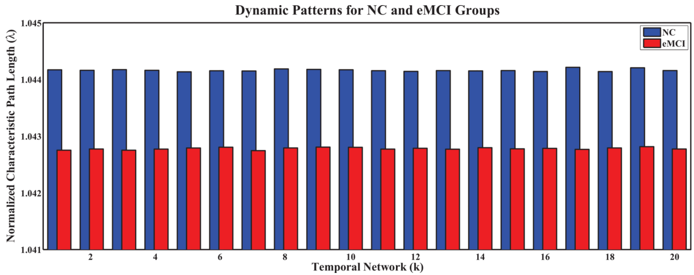
Fig. 8. Normalized characteristic path lengths of temporal networks for eMCI and NC groups with s = 2 and N = 90 .
