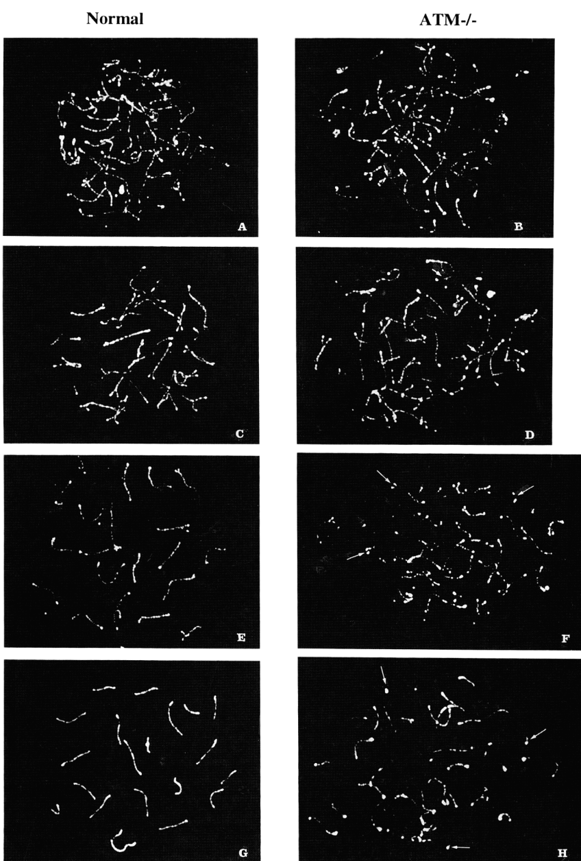
Figure 2. Comparison of progressively later zygotene and pachytene stages of normal spermatocytes (left) and ATM^{-/-} spermatocyte (right). (A,C) Normal zygotene nuclei stained with the Cor1 antibody showing progressive synapsis of bivalents from distal to proximal ends. (B,D) Similar stages of nuclei in ATM^{-/-} spermatocytes showing interstitial initiation of synapsis indicated by arrows. (E,G) A very late normal zygotene nucleus (E) with synapsis nearly complete and a normal mid-pachytene nucleus (G) with all autosomes fully synapsed. (F,H) Aberrant "pachytene" nuclei from ATM^{-/-} spermatocytes. Chromosome fragments are indicated with arrows.
