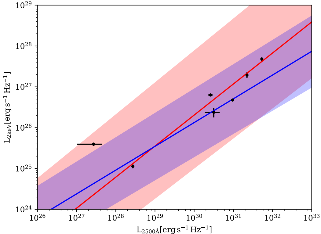
Figure 2. \log(L_{2500\text{\AA}}) vs. \log(L_{2\text{keV}}) for our seven sources. Error bars represent propagated 1\sigma uncertainties in optical fluxes, and 90% confidence intervals for X-ray fluxes. In red is the relation from Eq. 6 of Lusso et al. (2010) and in blue is the relation for the main sample from Table 2 of Lusso & Risaliti (2016). The shaded regions represent 1\sigma deviations from the mean relation.
