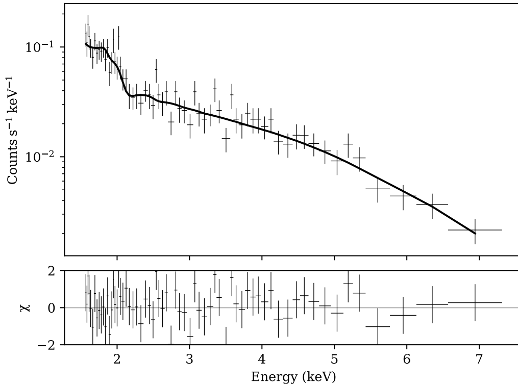
Figure 1. Chandra X-ray spectrum and best fit model for PG 1302-102, which is also typical of the other six sources in our sample. The plotted observed energies correspond to rest-frame 2-10 keV for the redshift of PG 1302-102. Error bars show 1\sigma confidence intervals. The source is well detected, and the spectrum is well-fit by a simple power-law model with the appropriate Galactic extinction for the source position.
