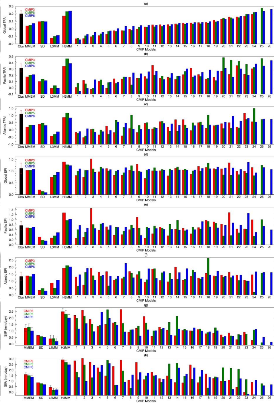
Figure 3. The global (a), Pacific (b) and Atlantic (c) tropical precipitation asymmetry indices (TPAIs) (a–c), the global (d), Pacific (e), and Atlantic (f) equatorial precipitation indices (EPIs) (d–f), the southern ITCZ index over the Pacific (SIIP, g) and the southern ITCZ index over the Atlantic (SIIA, h) from observations (wide black bars, none for g and h), multi-model ensemble means (MMEMs), standard deviations (SDs), lowest-3-model means (L3MMs), highest-3-model means (H3MMs), and all individual CMIP models (narrow bars). For all wide and narrow bars, red bars denote CMIP3 models, green bars for CMIP5 models, and blue bars for CMIP6 models. Their actual numerical values are listed in Table S2. The model numbers on the horizontal axis are the same model numbers listed in Table S1 and sorted in an ascending order by the global TPAI values shown in 3a and Table S2 for CMIP3, CMIP5 and CMIP6 models, respectively.
