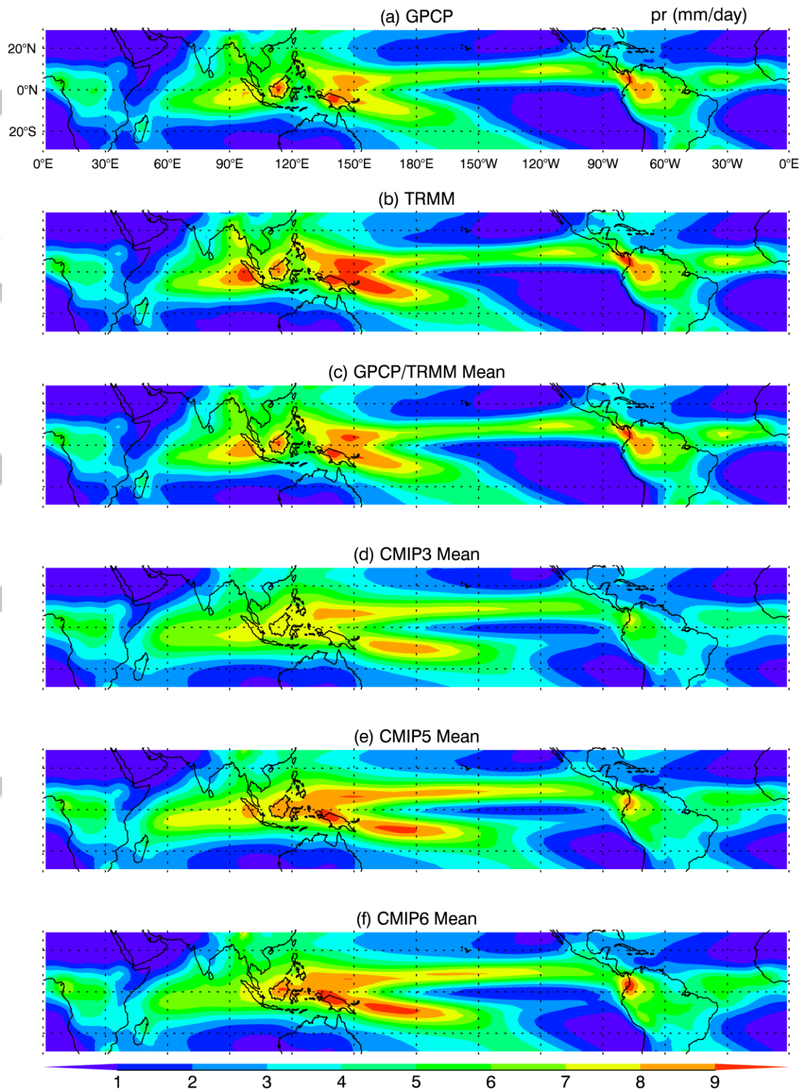
Figure 1. Long-term annual mean precipitation ( \text{mm day}^{-1} ) over the global tropics ( 30^{\circ}\text{S} – 30^{\circ}\text{N} ) from (a) GPCP, (b) TRMM, (c) GPCP/TRMM Mean, (d) CMIP3 multi-model ensemble mean (MEM), (e) CMIP5 MEM, and (f) CMIP6 MEM.
