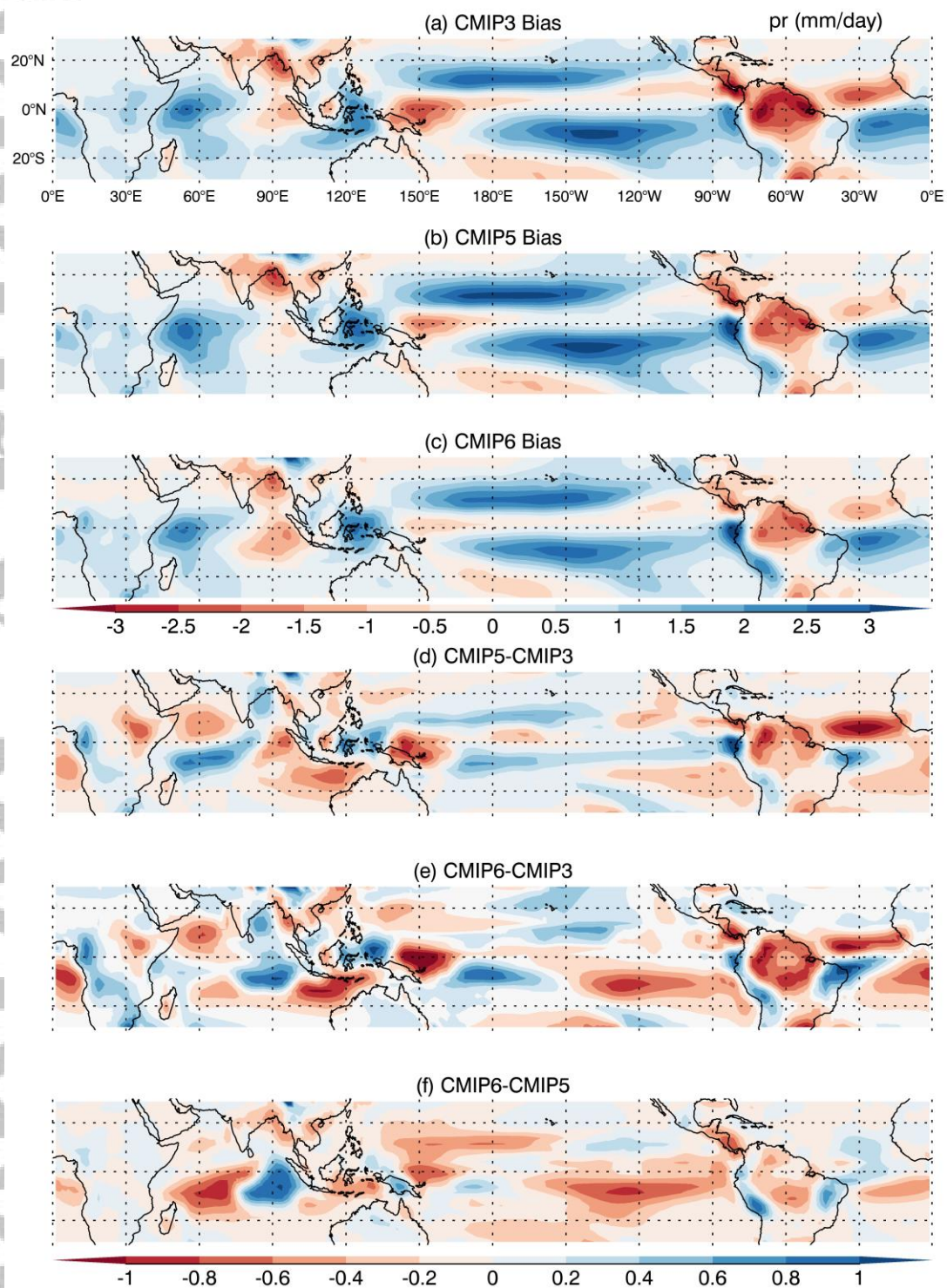
Figure 2. Long-term annual mean precipitation bias (model–observation, \text{mm day}^{-1} ) over the global tropics ( 30^{\circ}\text{S} – 30^{\circ}\text{N} ) from (a) CMIP3 MEM, (b) CMIP5 MEM, and (c) CMIP6 MEM. Difference of the absolute long-term precipitation bias over the global tropics ( 30^{\circ}\text{S} – 30^{\circ}\text{N} ) among generations of CMIP models: (d) CMIP5–CMIP3, (e) CMIP6–CMIP3, and (f) CMIP6–CMIP5.
