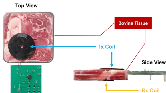
Fig. 2: In Vitro Experimental Setup. Photo of experimental setup for in vitro analysis of power transfer efficiency over various distances and misalignment levels. A segment of bovine tissue containing a mixture of muscle, adipose, and bone was placed in between the two coils to mimic the environment of the body.
