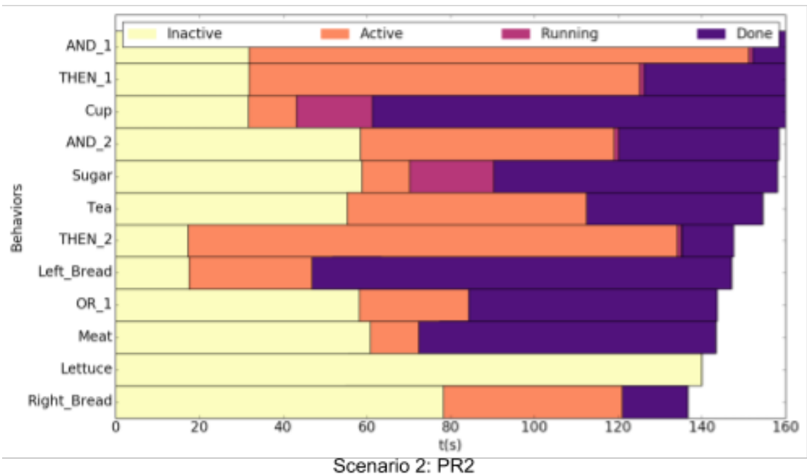
FIGURE 4.10: The timing diagrams of the second tea-time task scenario on the PR2 and the Baxter. The top image is the timing diagram for the Baxter and the bottom image is the timing diagram for the PR2. These diagrams represent the times at which the state of a node in a given task tree changed. Within each graph, each row corresponds to a behavior node named as its corresponding object. The horizontal axis is increasing time.
