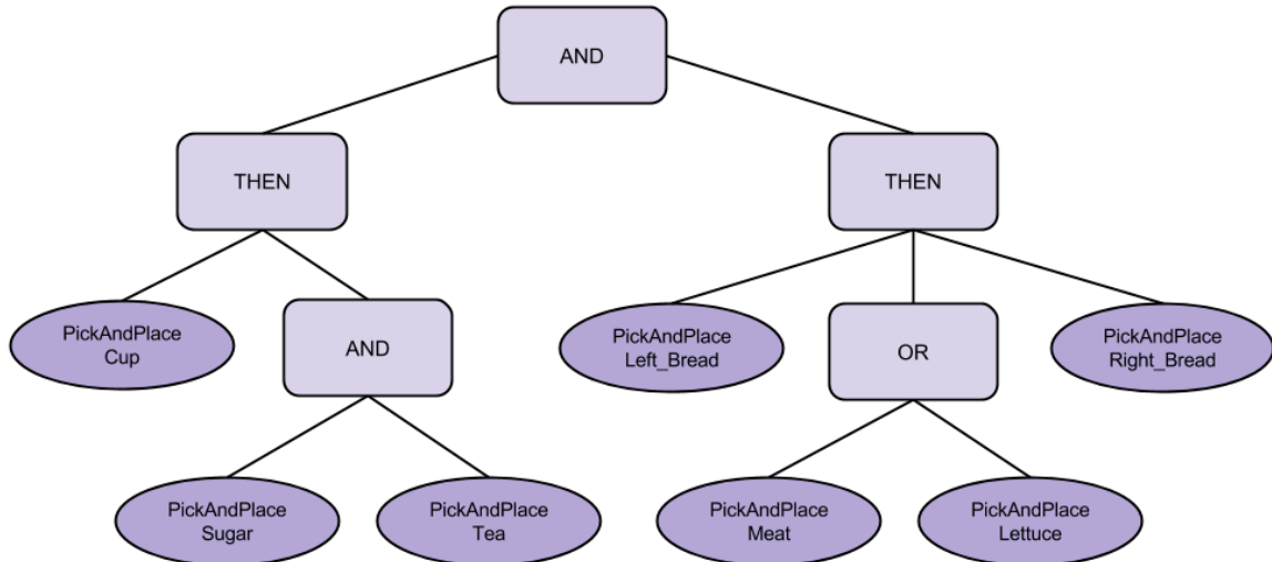
FIGURE 3.1: The full task structure of the tea-time task experiment. Both robots have an identical copy of this task tree. The lighter purple nodes represent the goal nodes of the task structure and the darker purple nodes represent the behavior nodes.
