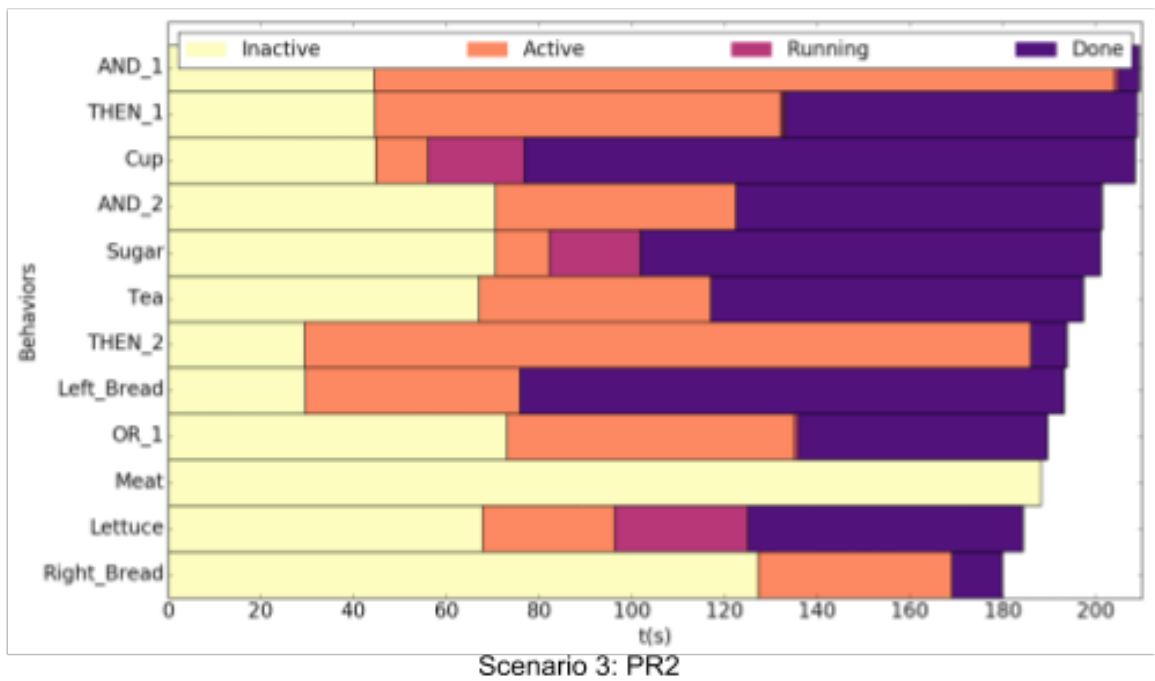
FIGURE 4.11: The timing diagrams of the third tea-time task scenario on the PR2 and the Baxter. The top image is the timing diagram for the Baxter and the bottom image is the timing diagram for the PR2. These diagrams represent the times at which the state of a node in a given task tree changed. Within each graph, each row corresponds to a behavior node named as its corresponding object. The horizontal axis is increasing time.
