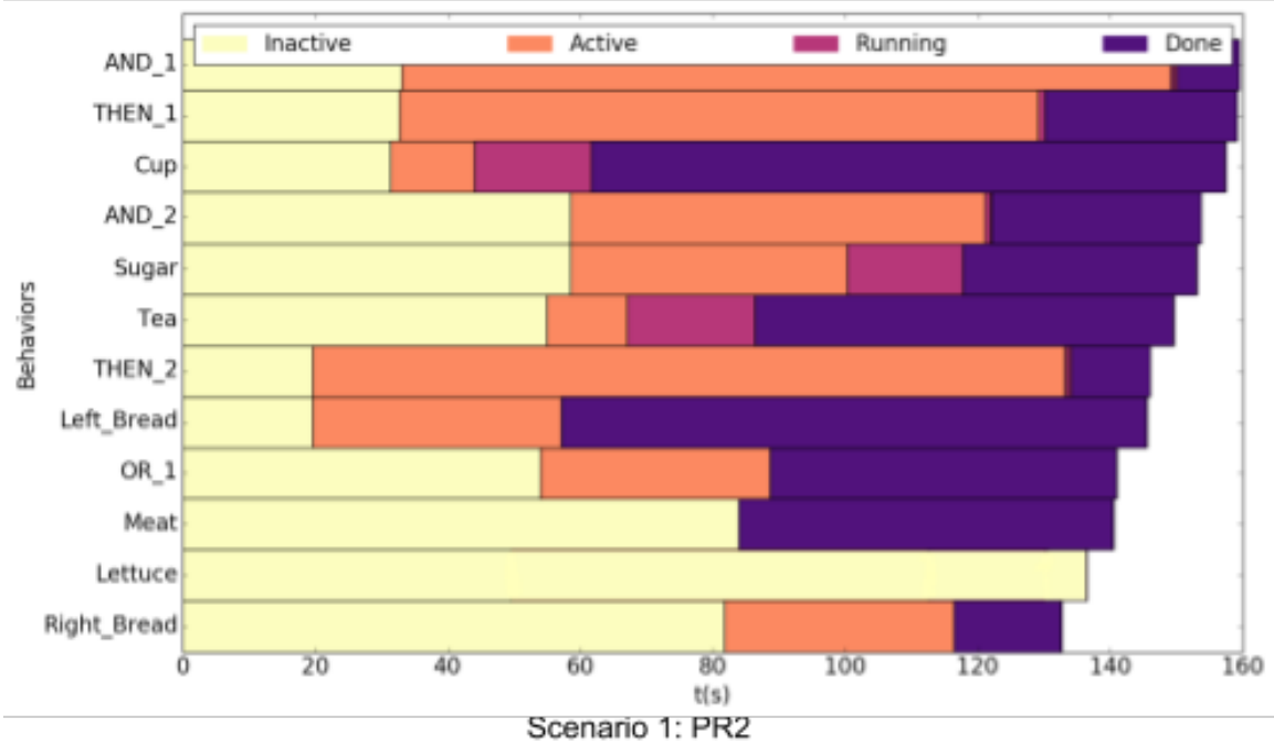
FIGURE 4.9: The timing diagrams of the first tea-time task scenario on the PR2 and the Baxter. The top image is the timing diagram for the Baxter and the bottom image is the timing diagram for the PR2. These diagrams represent the times at which the state of a node in a given task tree changed. Within each graph, each row corresponds to a behavior node named as its corresponding object. The horizontal axis is increasing time.
