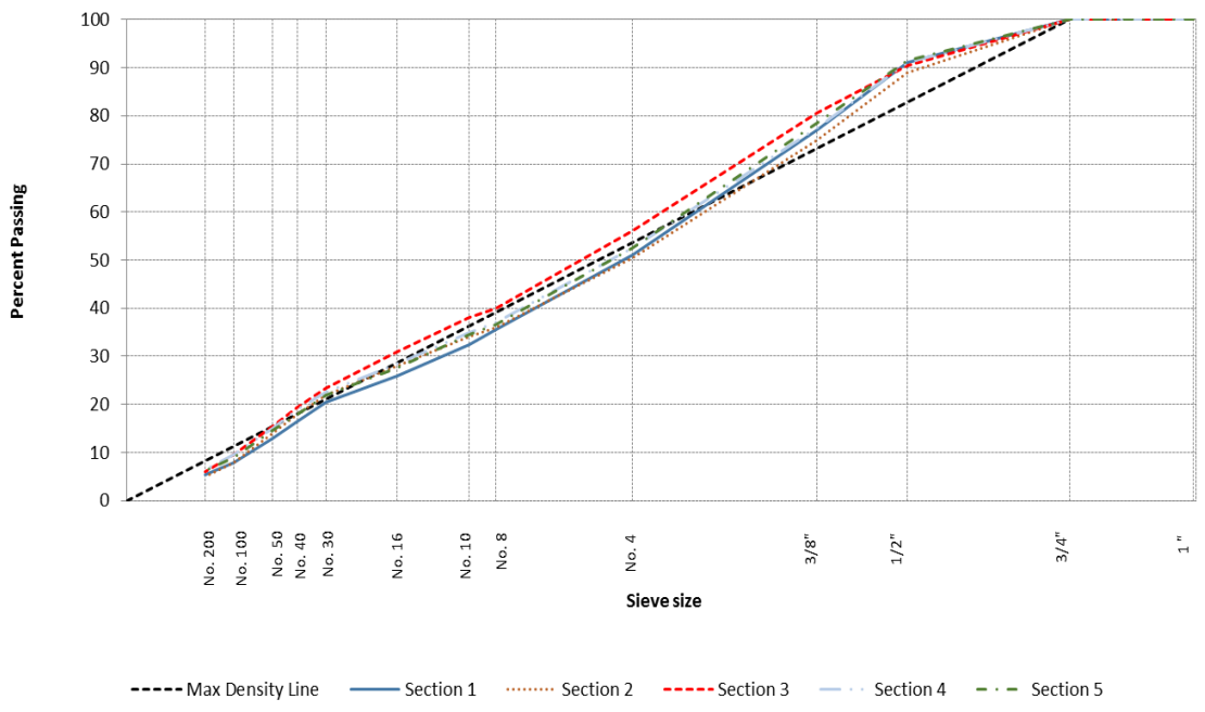
Figure 9. 8. Hot Mix Asphalt Aggregate Gradation from QC Samples
