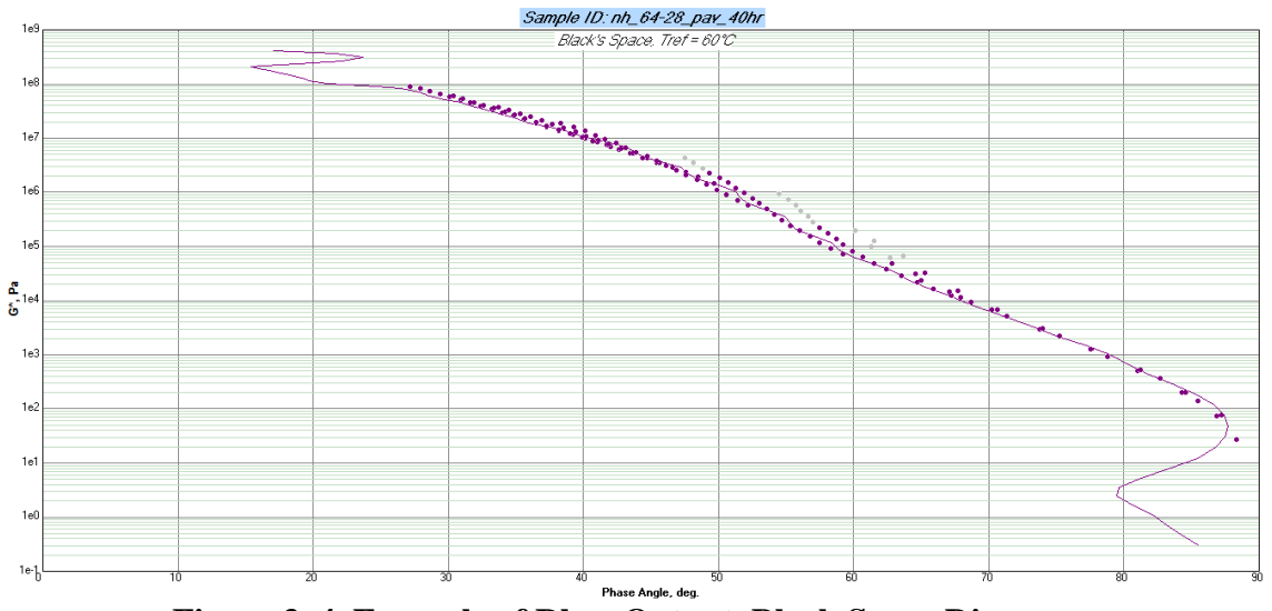
Figure 3. 4. Example of Rhea Output, Black Space Diagram
