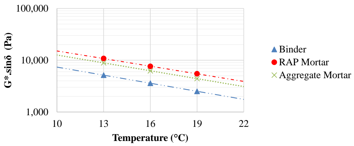
Figure 3. 10. Intermediate Temperature Properties for PG 64-28P
