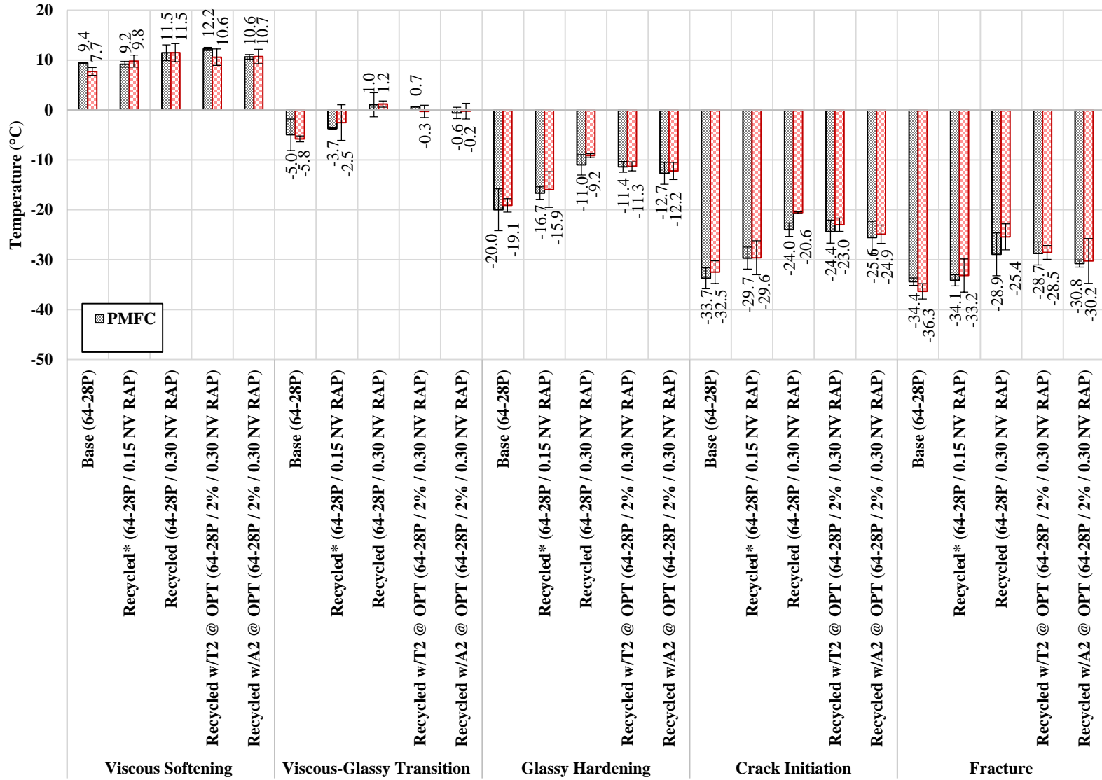
Figure 7. 16. UTSSST Critical Temperature Measures for Nevada Field Sections, PMFC and RPMLC
