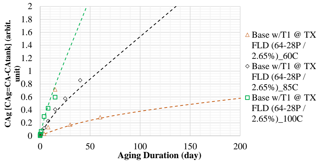
Figure 10. 10. Oxidation of Base 64-28P w/T1 @ TX FLD after 60, 85, and 100°C Oven Aging
