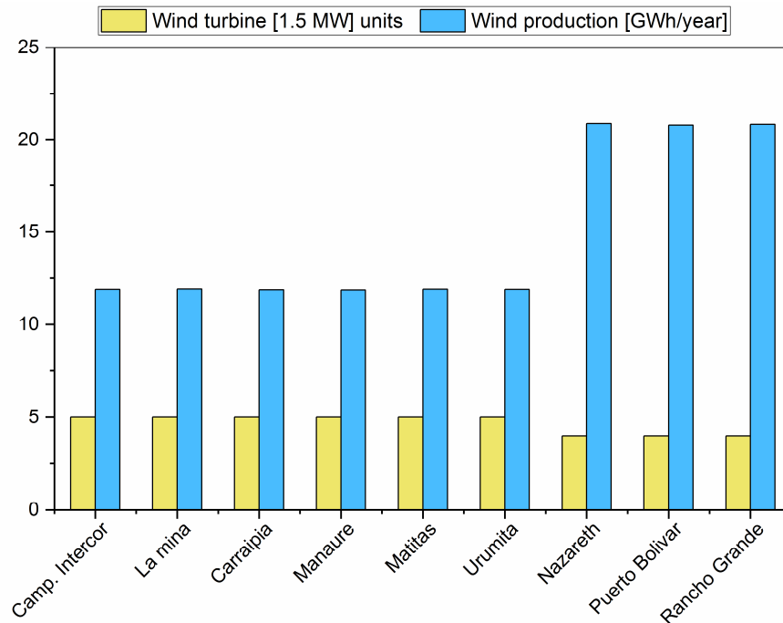
Figure 8. Comparison between the number of wind turbines and the annual energy production for each location.
