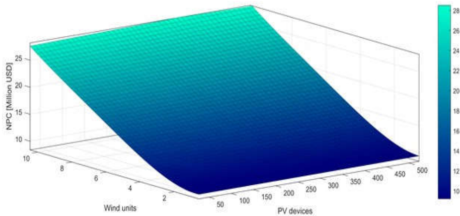
Figure 12. Polynomial regression for NPC (Rancho Grande).
