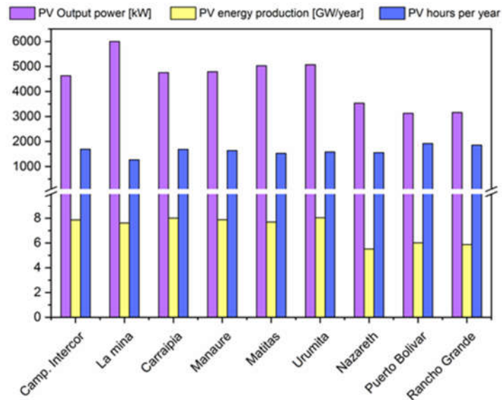
Figure 7. Comparison between the rated power and energy production for the photovoltaic (PV) system.
