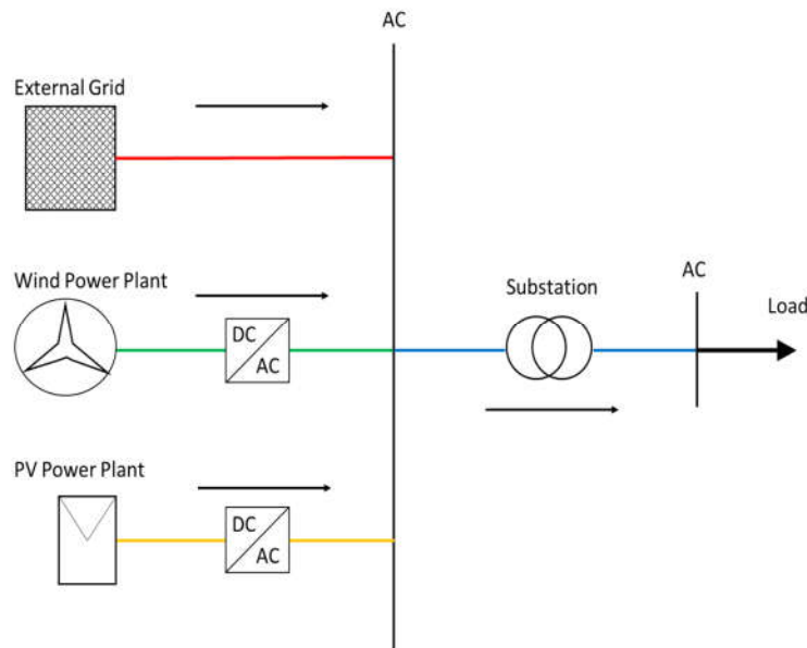
Figure 3. Proposed energy system scheme.
