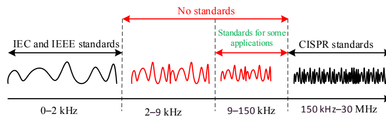
Fig. 1: Harmonic and conducted emission frequency ranges classification.
