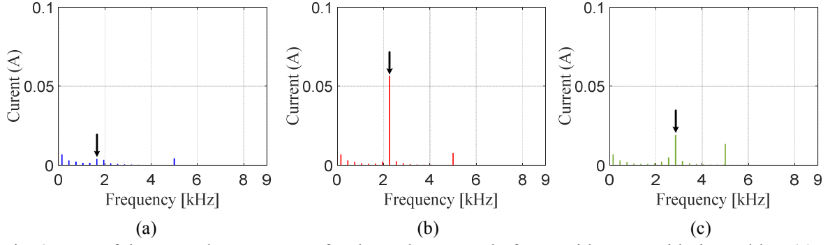
Fig. 9: FFT of the ground current i_{g-grid} for the real system platform; without considering cables. (a) Normal case, (b) decreasing L_{cm} to 60% of L_{cm} , (c) decreasing C_{yAC} to 40% of C_{yAC} .
