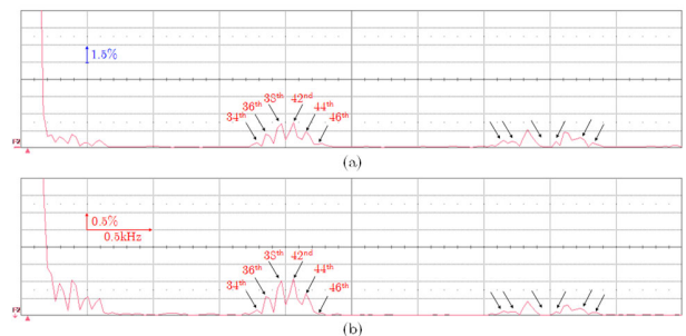
Fig. 21. The harmonics spectrum of proposed topology when the third cell is shaded in, (a) the output voltage, and (b) current injected to the grid.
