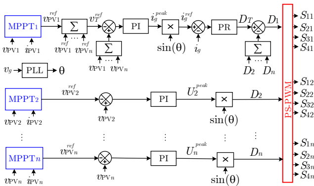
Fig. 5. The control structure adopted for the proposed cascaded H6 converter.
