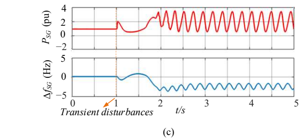
Fig. 17. Simulation results under the condition of H_{VSG1}=1.59 s, H_{VSG2}=1.59 s, H_{SG}=1.59 s, where the mode-adaptive control is applied to VSG1 and VSG2, and the system is unstable. (a) VSG1. (b) VSG2. (c) SG.
