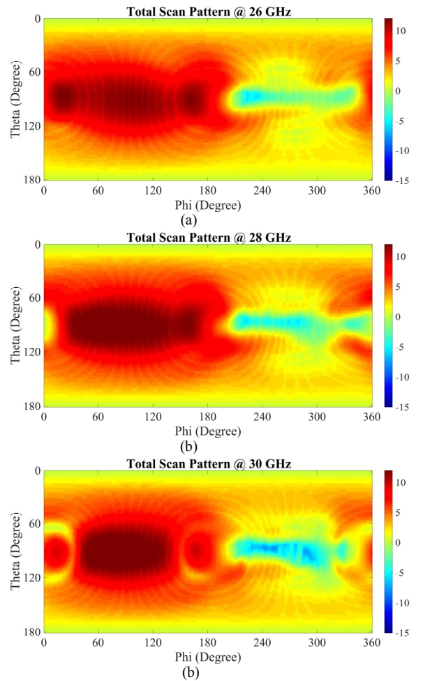
Fig. 6. The total scan pattern of antenna at different direction angle at (a) 26 GHz, (b) 28 GHz, (c) 30 GHz.
