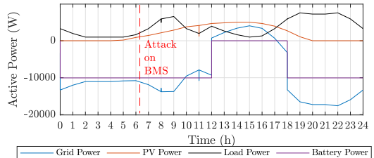
(b) Active power profile under MITM attack.
