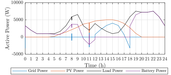
(a) Active power profile under normal conditions.
