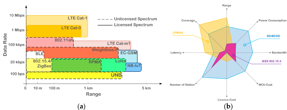
Figure 1. Communication technologies utilized in IoT applications: (a) Data rate versus range comparison of wireless technologies, (b) comparison of a low power wide area network (LPWAN) with IEEE 802.15.4 and 3G/4G/5G cellular communication technologies.
